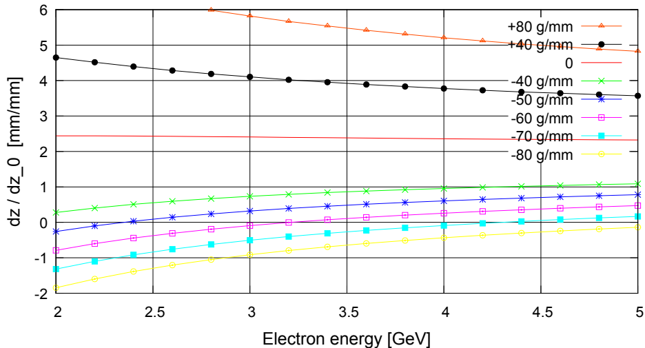
dz/dz_0 (no quad, and 7 quad gradients)
