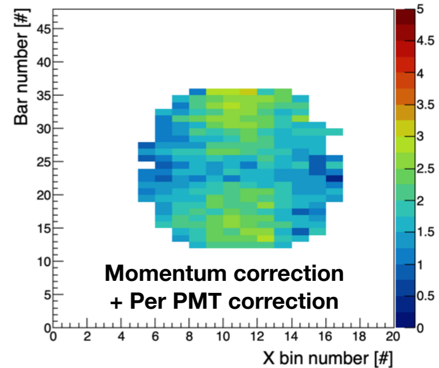
\pi/k separation at momentum [3.5-4] GeV/c beam data PMT Corrected
