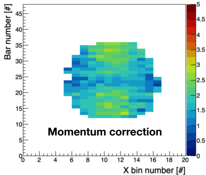
\pi/k separation at momentum [3.5-4] GeV/c beam data
