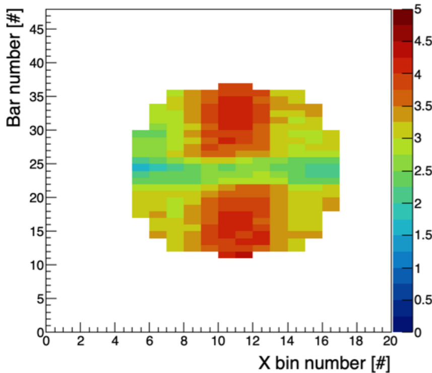
\pi/k separation at momentum [3.5-4] GeV/c simulation
