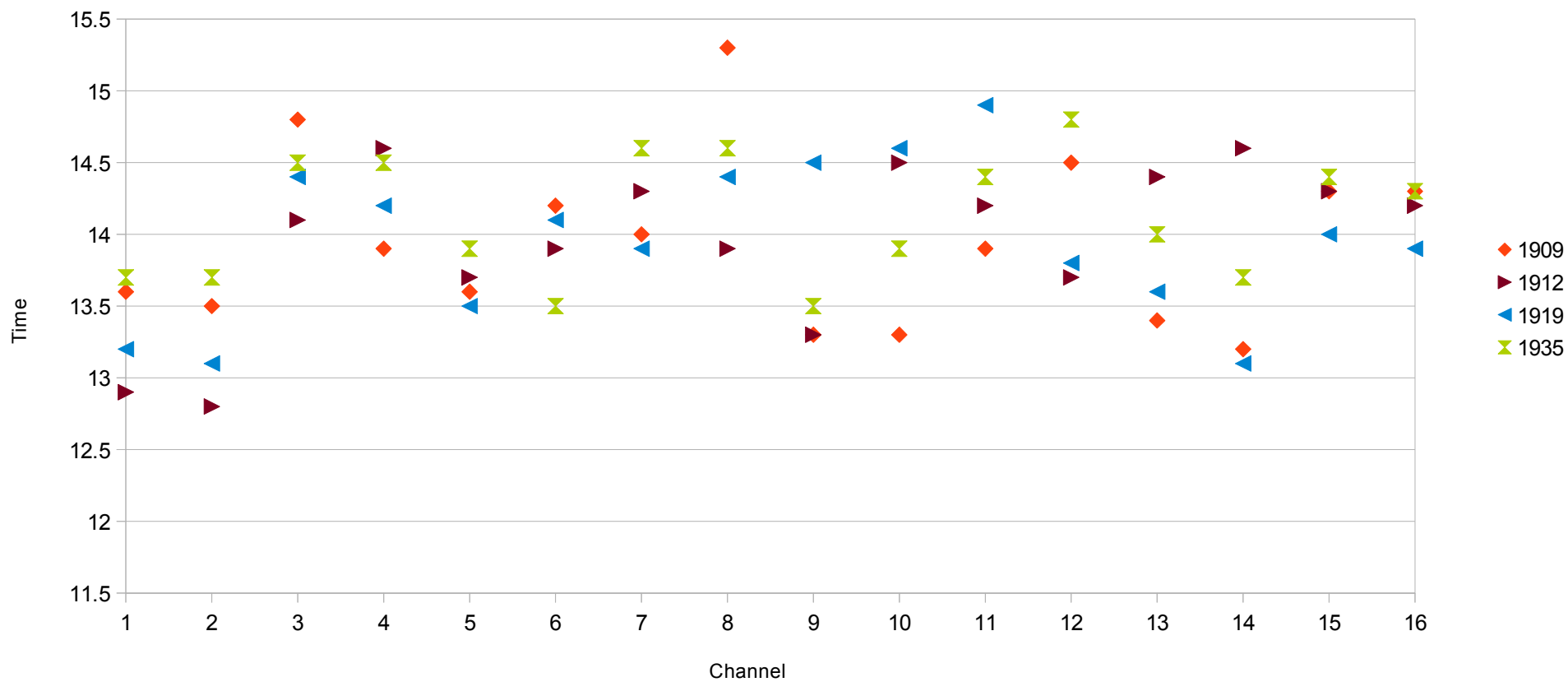
Rise Time
