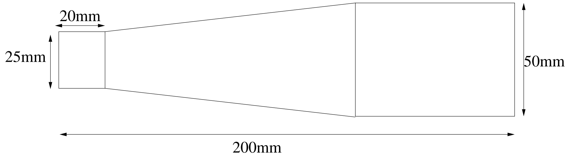
Top view
