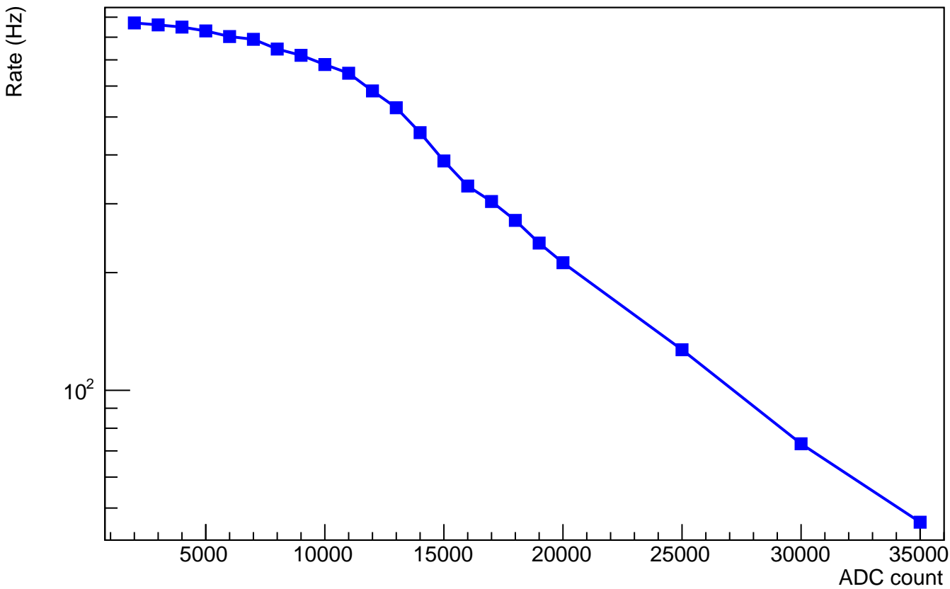
BCAL noise/cosmic
