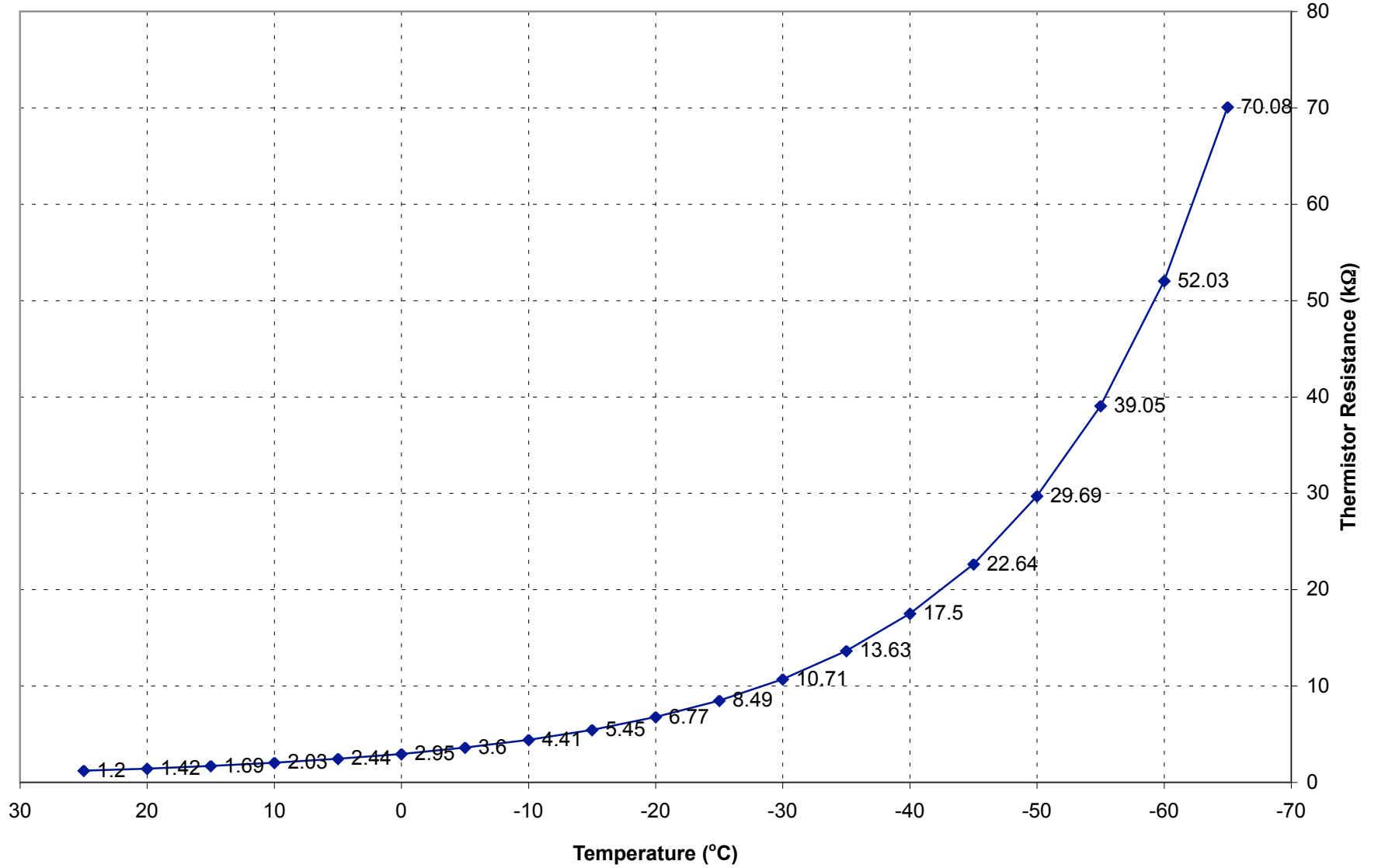
Thermistor Resistance Calibration Plot
