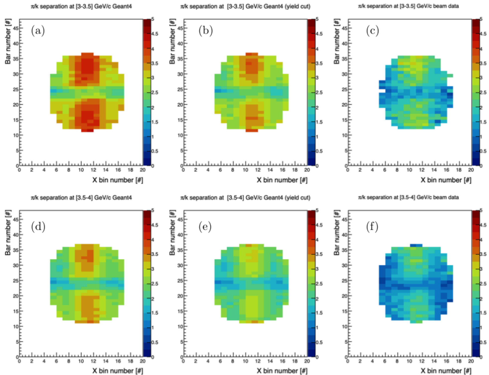
Figure 1.22: pion/kaon separation power maps (a) Simulation at momentum between 3-3.5 GeV/ c , (b) Simulation at momentum between 3-3.5 GeV/ c after photon cut, (c) Beam data at momentum between 3-3.5 GeV/ c , (d) Simulation at momentum between 3.5-4 GeV/ c , (e) Simulation at momentum between 3.5-4 GeV/ c after photon cut, (f) Beam data at momentum between 3.5-4 GeV/ c
