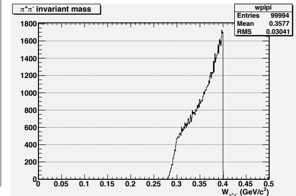
Generated signal plus \rho background (plot from Candace)
