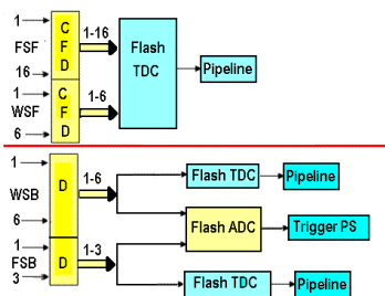
Figure 4: Sketch of the original proposed electronics.
