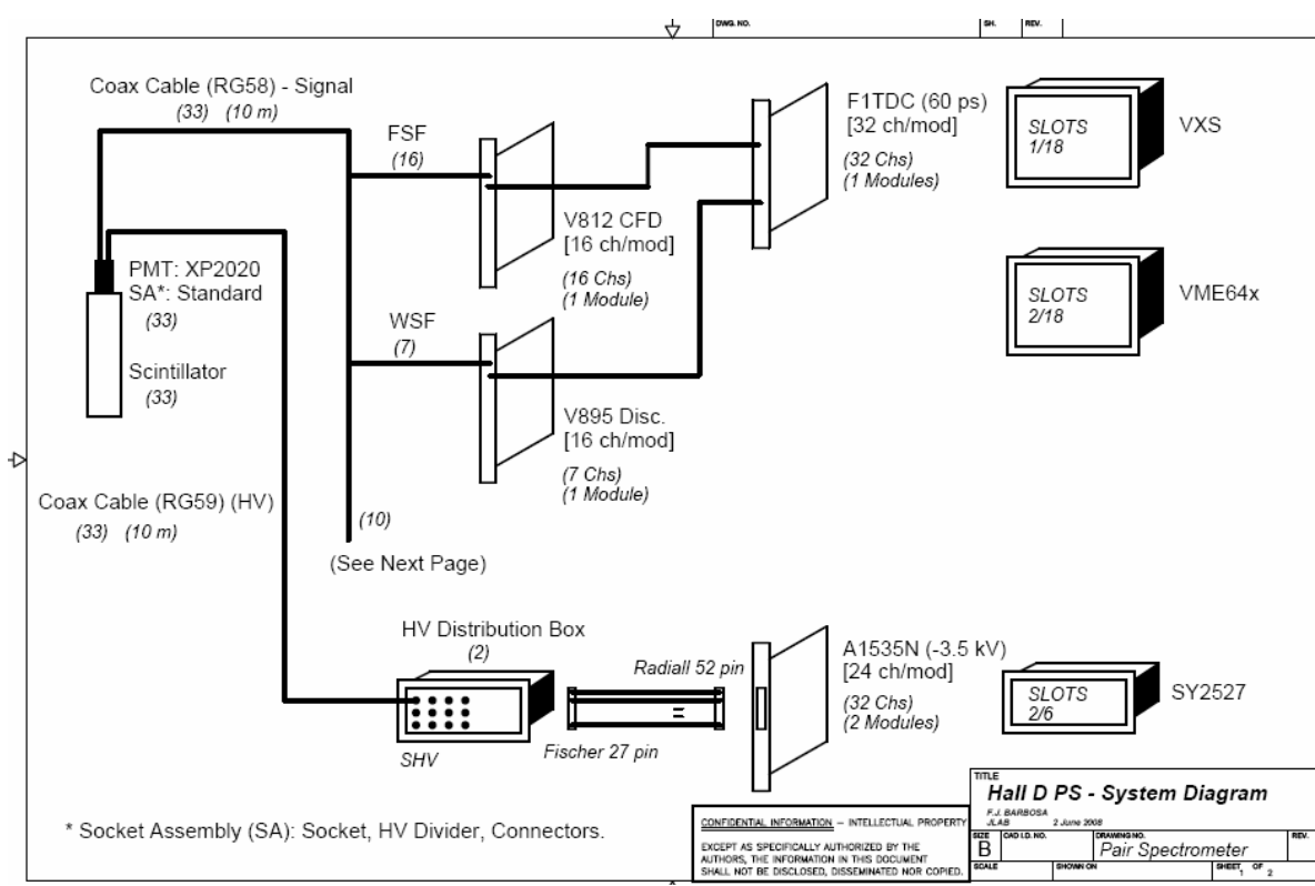
Figure 5: Readout scheme for the pair spectrometer.
