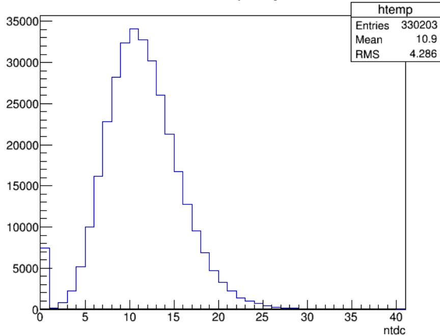
TAGM tdc multiplicity count
