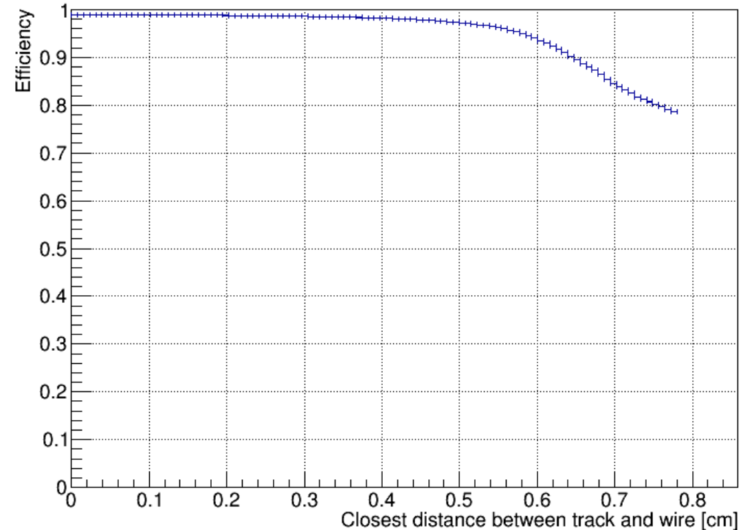
CDC Per Straw Efficiency Vs. DOCA
