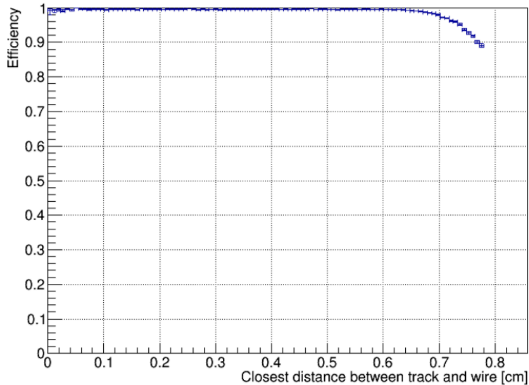
CDC Per Straw Efficiency Vs. DOCA
