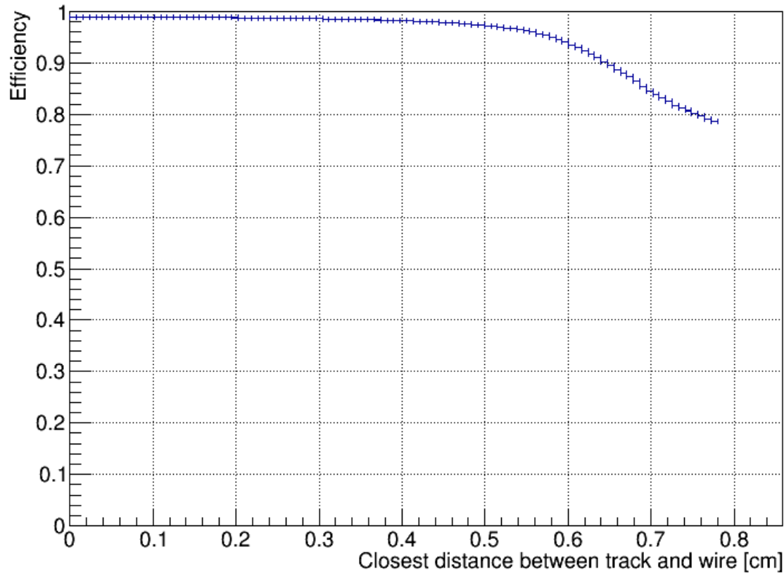
CDC Per Straw Efficiency Vs. DOCA
