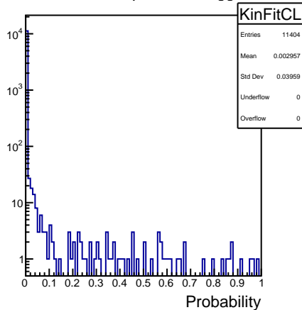
DSelector_Z2pi0_trees_bggen
