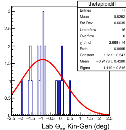
DSelector_Z2pi0_trees_bggen
