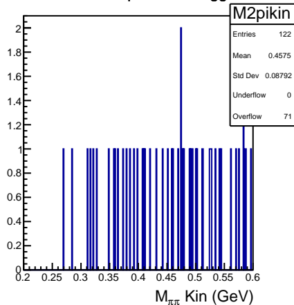
DSelector_Z2pi0_trees_bggen
