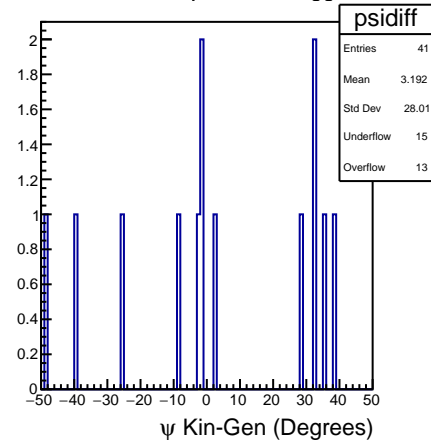
DSelector_Z2pi0_trees_bggen
