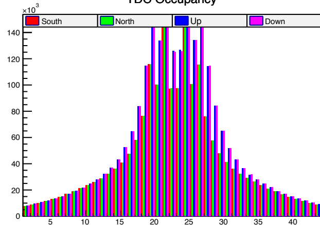
TDC Occupancy
