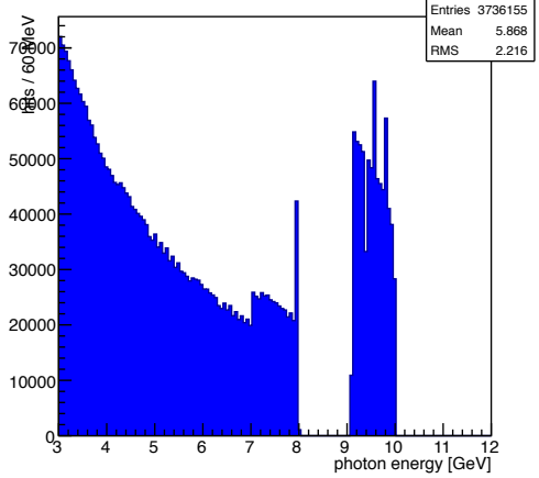
TAGH energy
