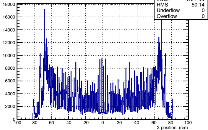
x (DBCALShower)
