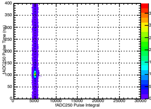
ST IADC250 Pulse Integral
