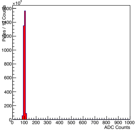
FCAL Pedestal (All Channels)
