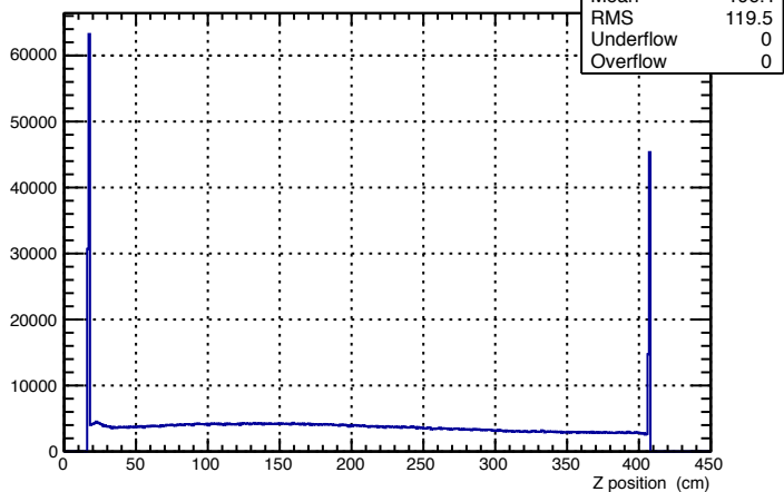
z (DBCALShower)
