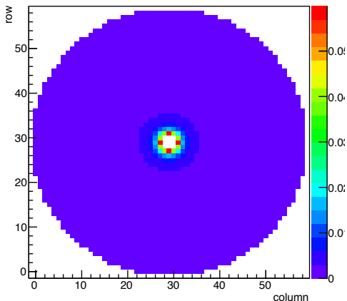
FCAL Hit Occupancy per Event
