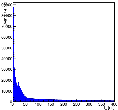
FCAL Cluster Energy Weighted Average Time
