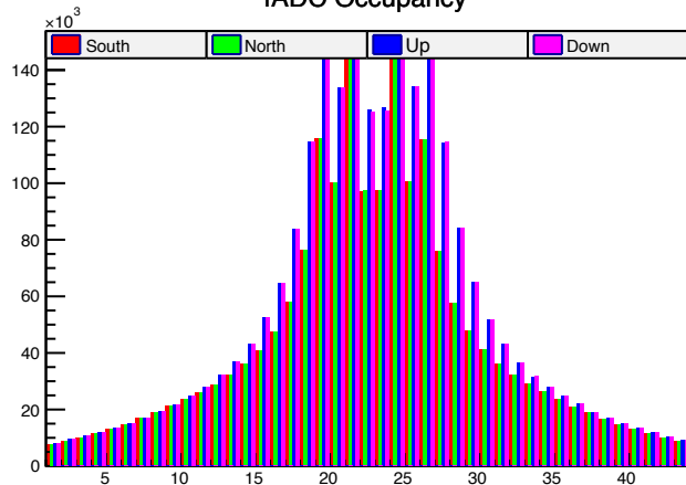
fADC Occupancy
