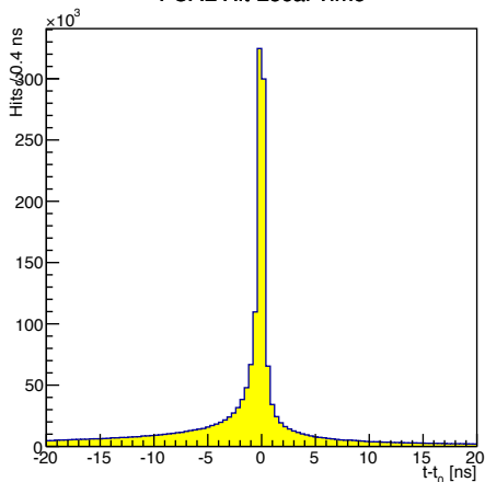
FCAL Hit Local Time
