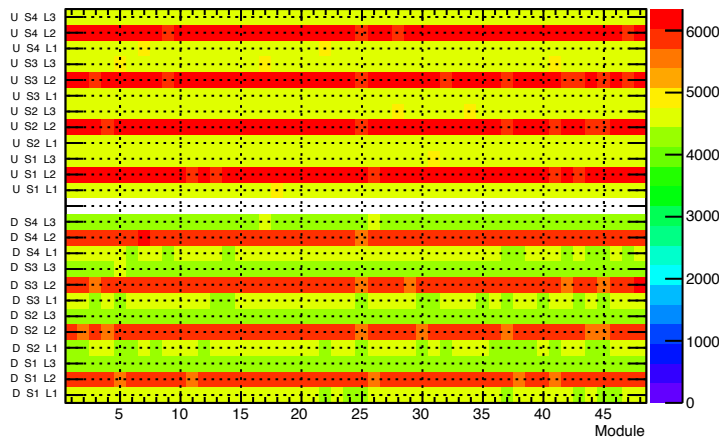
TDC occupancy (DBCALDigiTDCHit)
