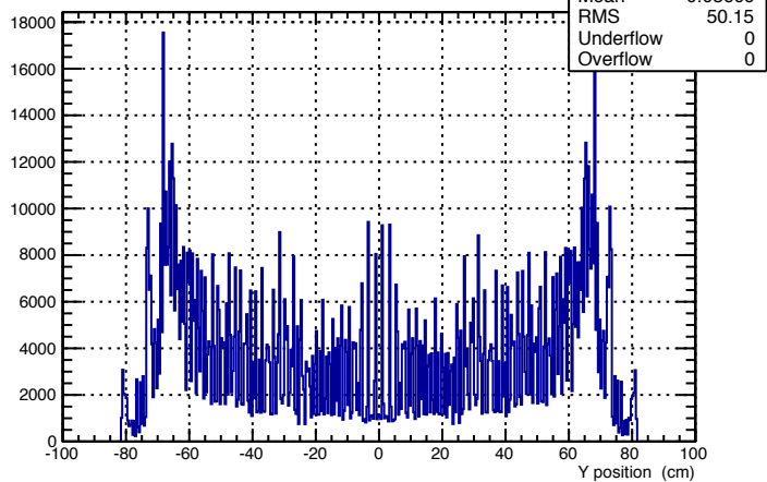
y (DBCALShower)
