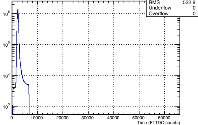
TDC Time (DBCALDigiTDCHit)
