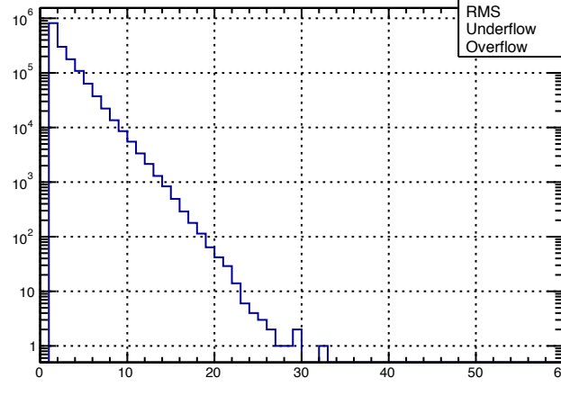
Number of Cells (DBCALCluster)
