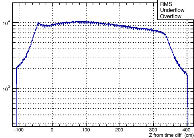
z (DBCALPoint)
