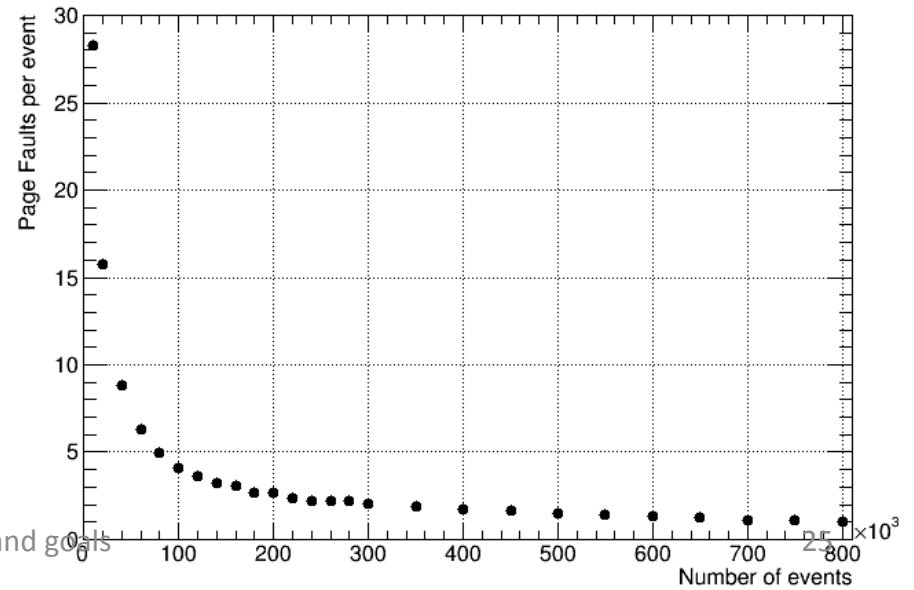
Page Faults/event
