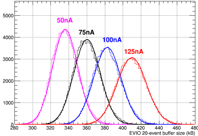
buffer size
