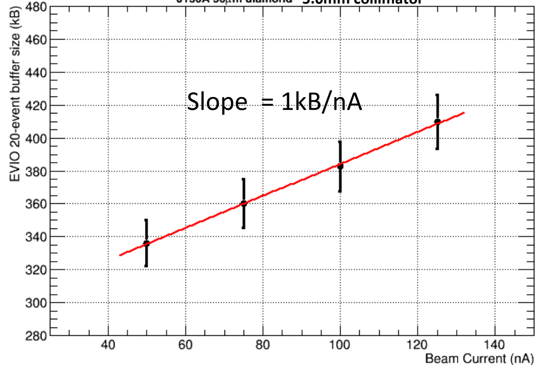
buffer size vs. beam current
