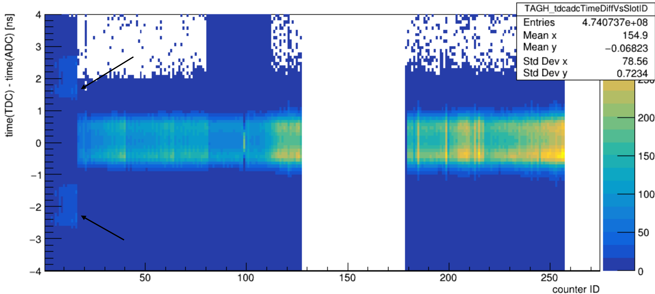
TAGH TDC-ADC time difference vs. counter ID
