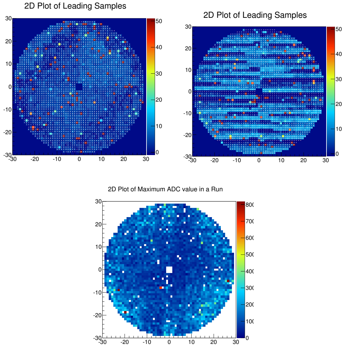
Figure 2: Top Left: Led Pulser, Top Right: Base Pulser Bottom: LED Pulser
