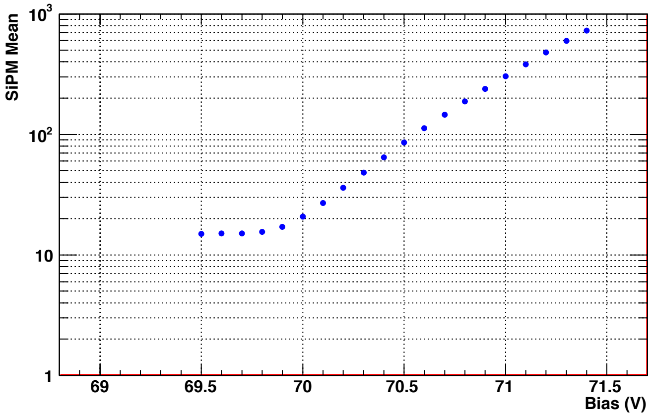
SiPM 10 Uncorrected breakdown n (Ham. Vop=70.79 @ 25C)
