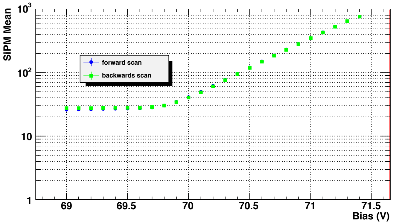
SiPM 2 Uncorrected breakdown (Ham. Vop=70.72 @ 25C)
