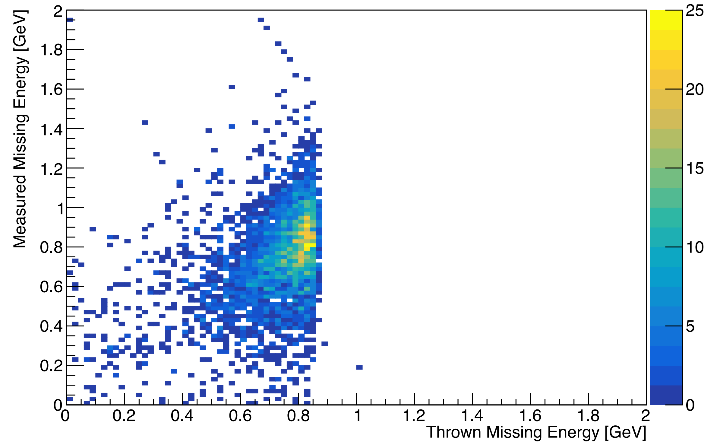
4\text{He}(\gamma, \rho^- pp) GCF Simulation
