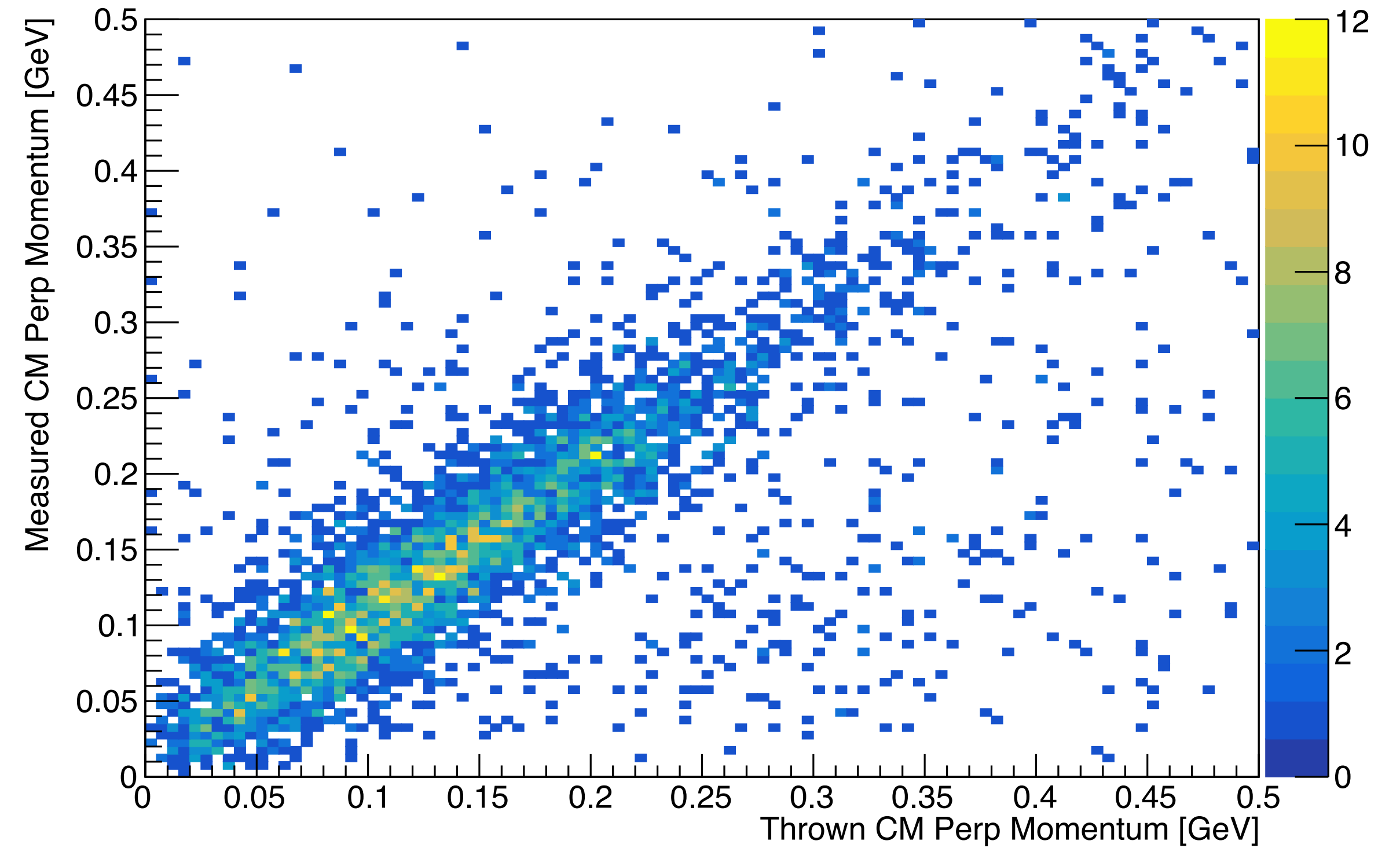
4\text{He}(\gamma, \rho^- pp) GCF Simulation
