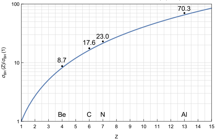
Bethe-Heitler total XS Ratios - Tsai, Eq. (3.61)
