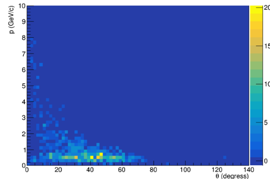
Proton Momentum v. Theta
