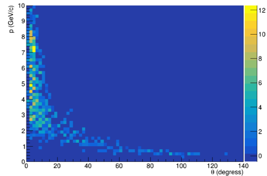
\text{Pi}^- Momentum v. Theta
