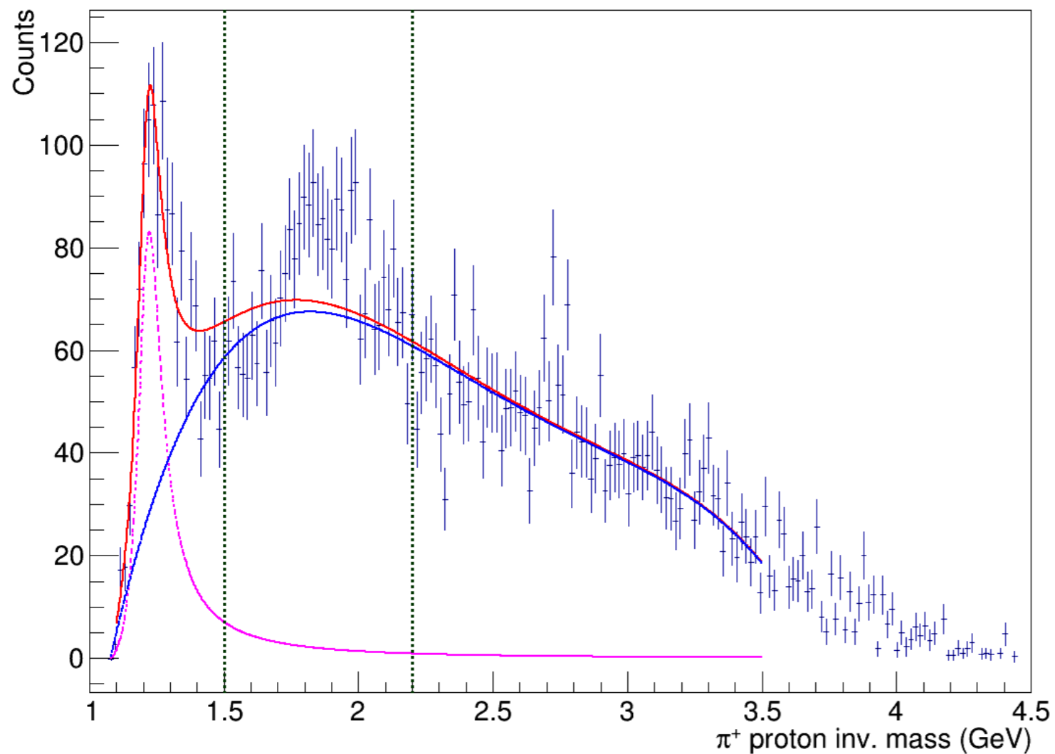
\text{Pi}^+ Proton Mass Spectrum
