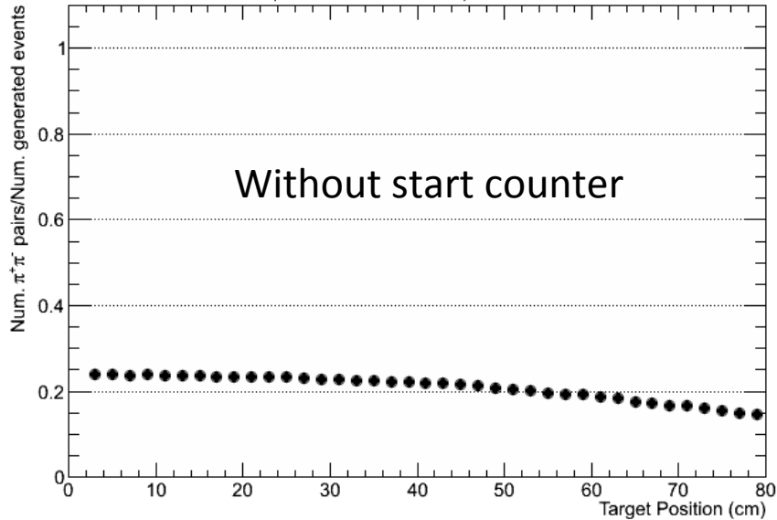
Rough efficiency vs. target position December 7, 2012 DL svn revision 9877 100k \pi^+ \pi^- events generated
