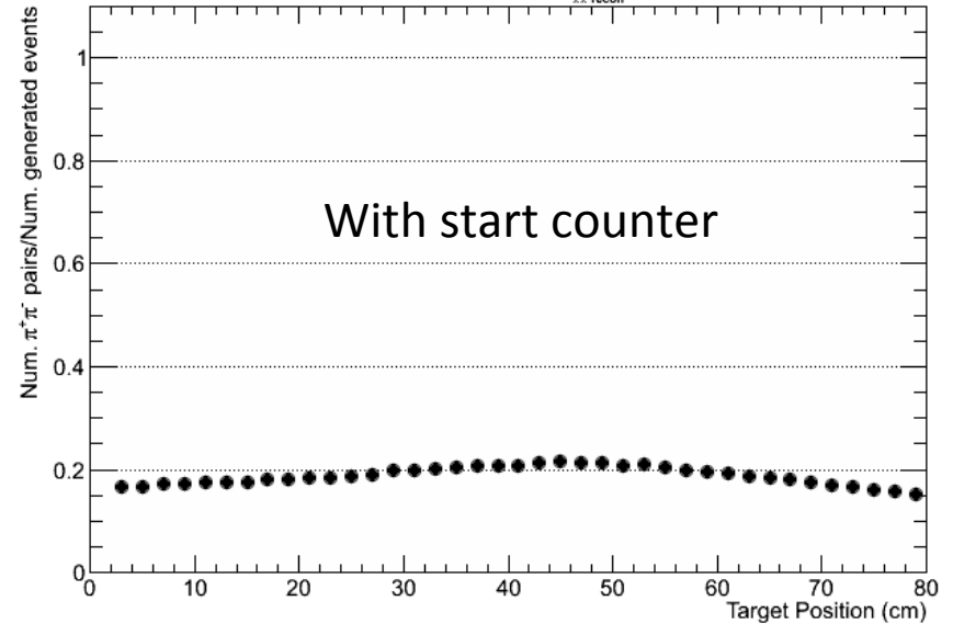
Rough efficiency vs. target position November 29, 2012 DL svn revision 9938 100k \pi^+ \pi^- events generated
