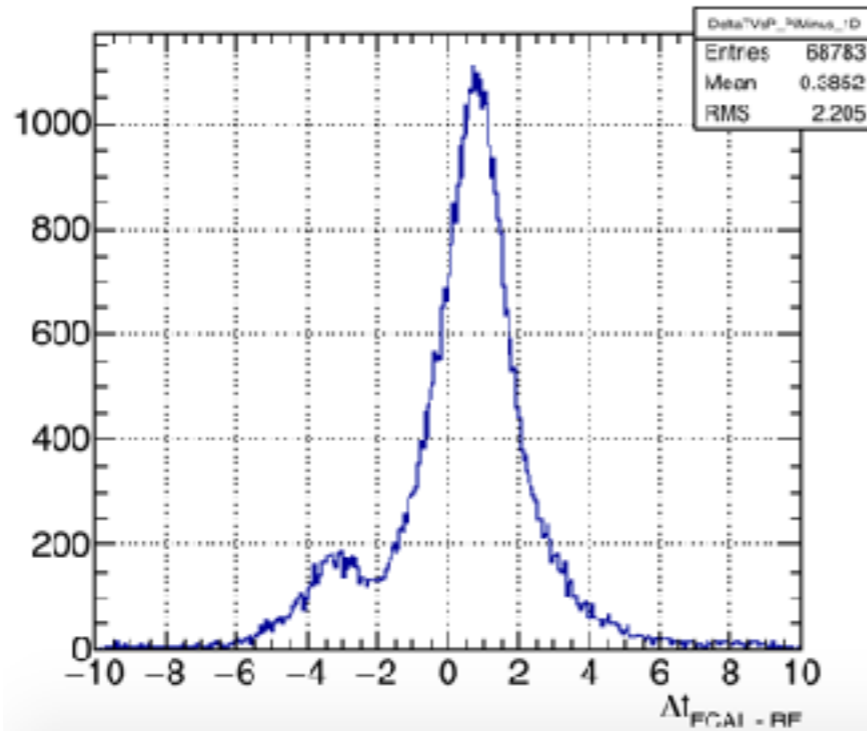
FCAL \pi^- Candidates
