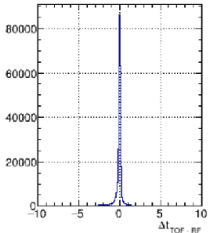
TOF \pi^- Candidates
