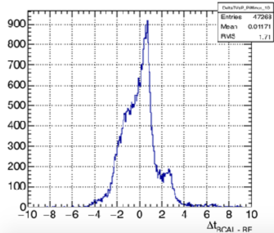
BCAL \pi^- Candidates
