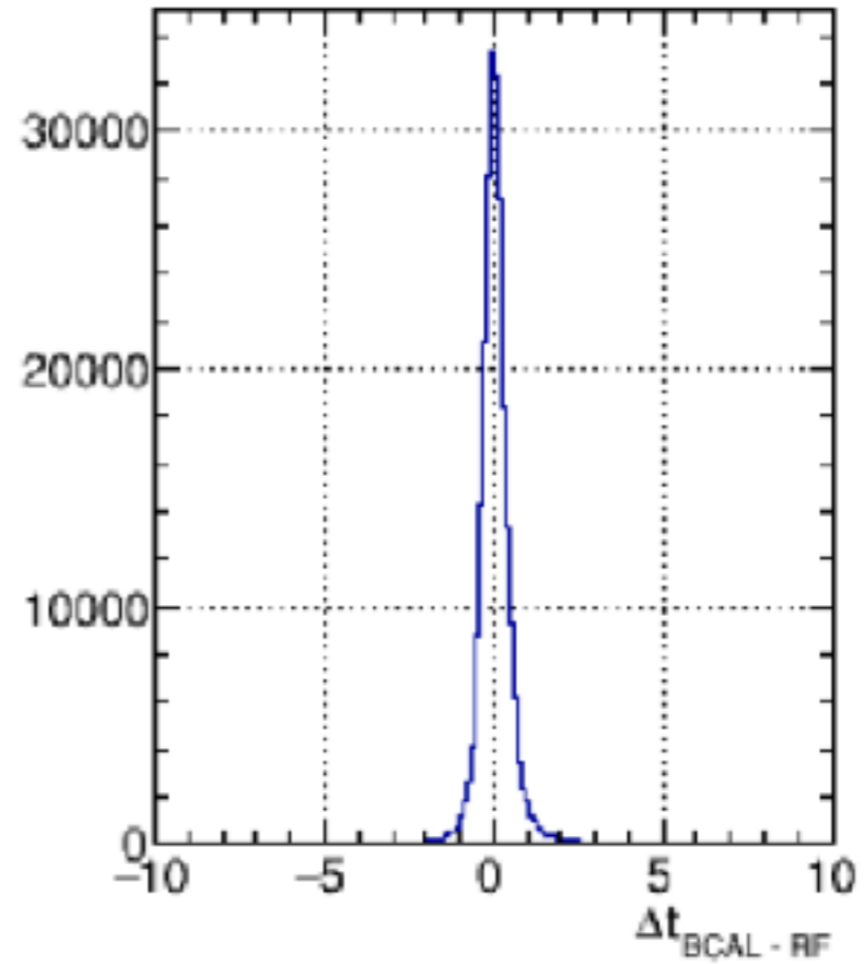
BCAL \pi^- Candidates
