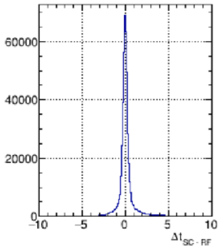
SC \pi^- Candidates
