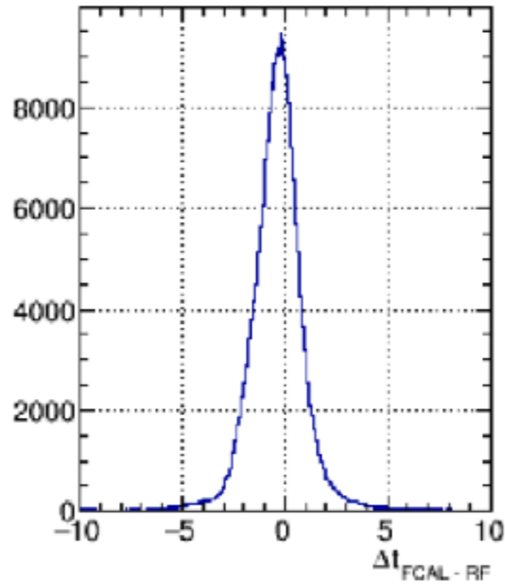
FCAL \pi^- Candidates
