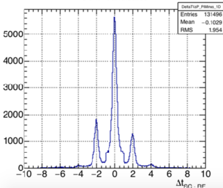
SC \pi^- Candidates
