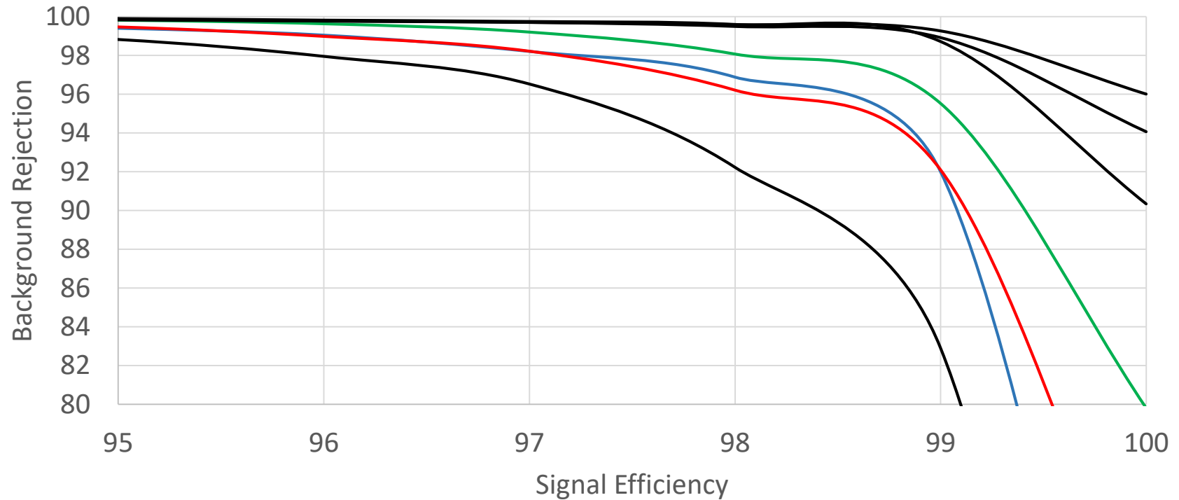
Signal vs. Background Efficiency, 8 detectors, Varying Geometries
