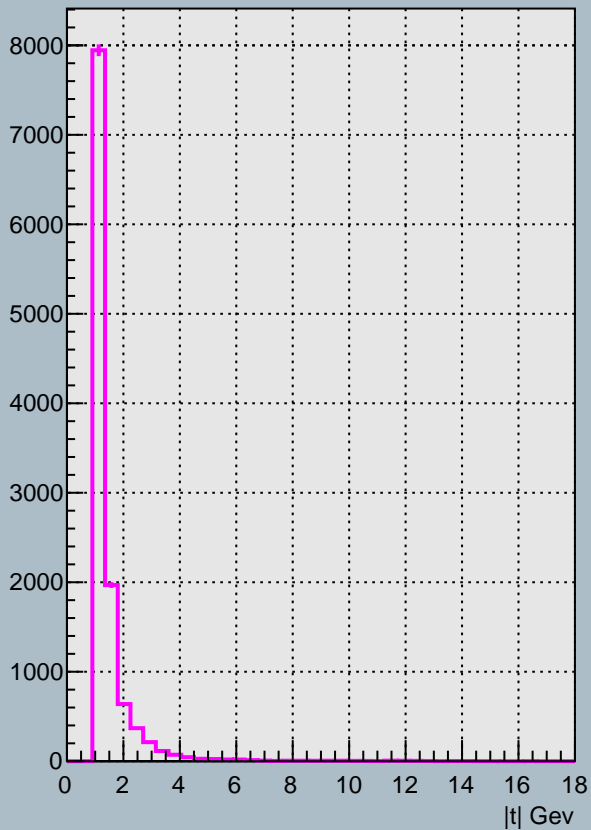
|t| distribution simulation
