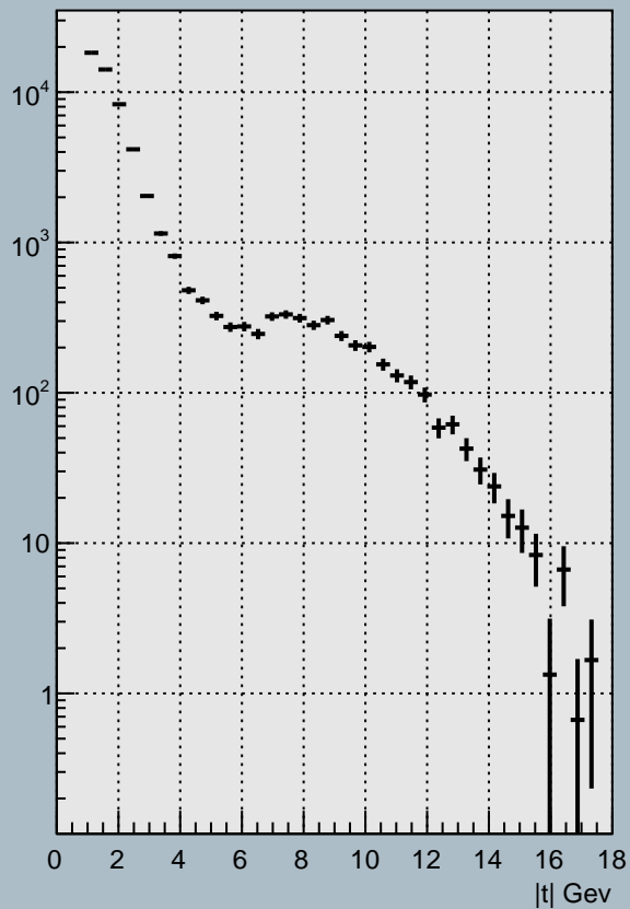
|t| distribution data
