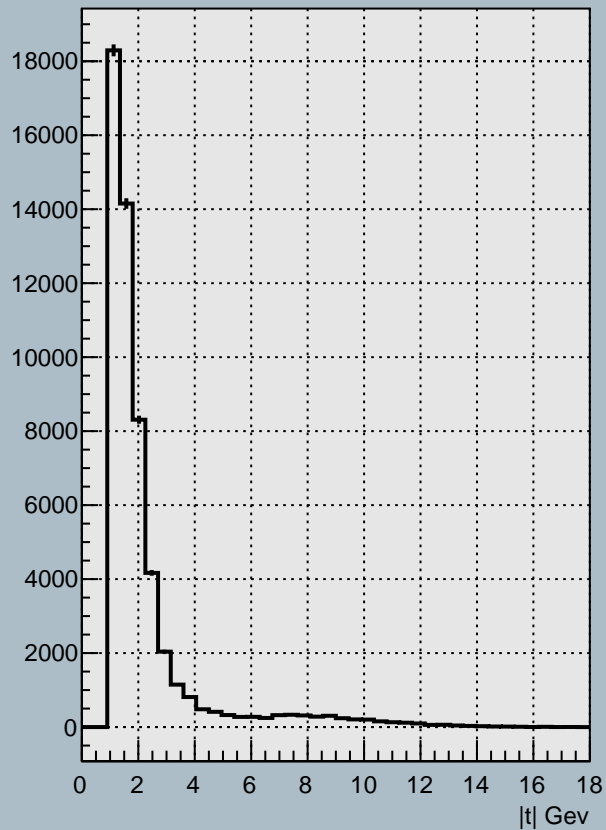
|t| distribution data
