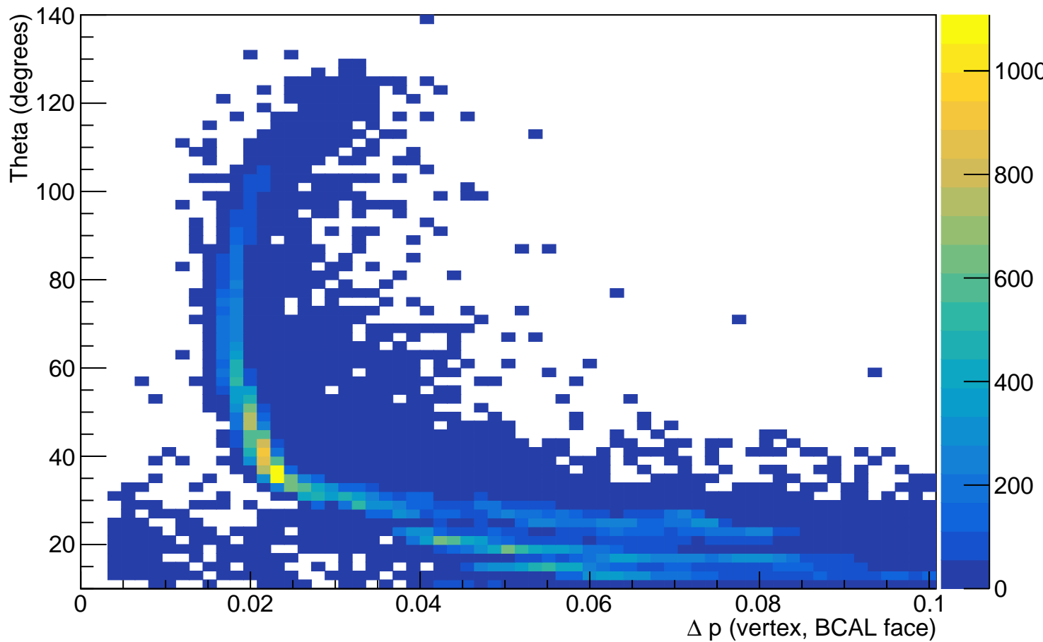
fractional change between momentum of e^-_{\text{track}} at vertex and BCAL face
