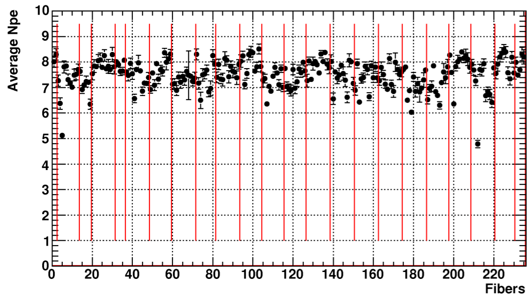
8th shipment: Npe with PMT
