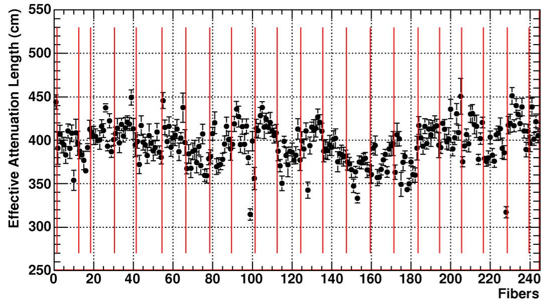
8th shipment: Attenuation Length with Photodiode
