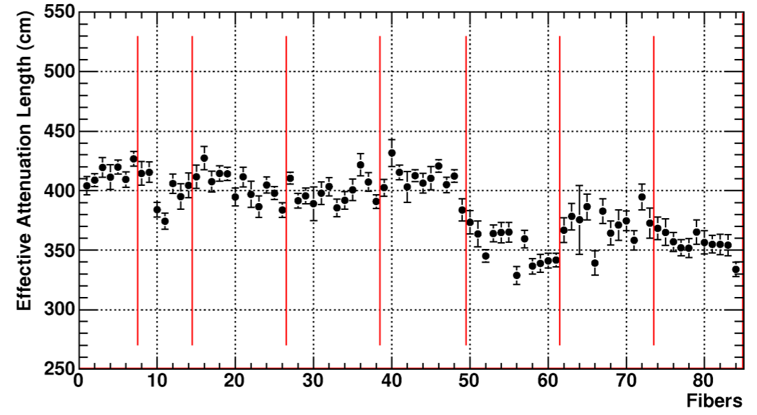
9th shipment: Attenuation Length with Photodiode
