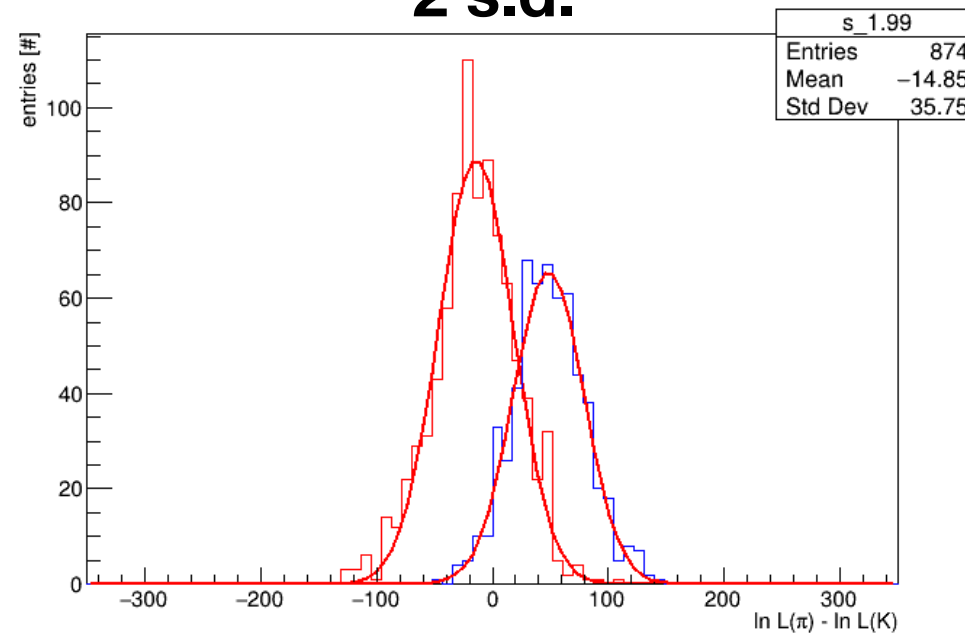
Simulated Cherenkov PDF using particle gun
