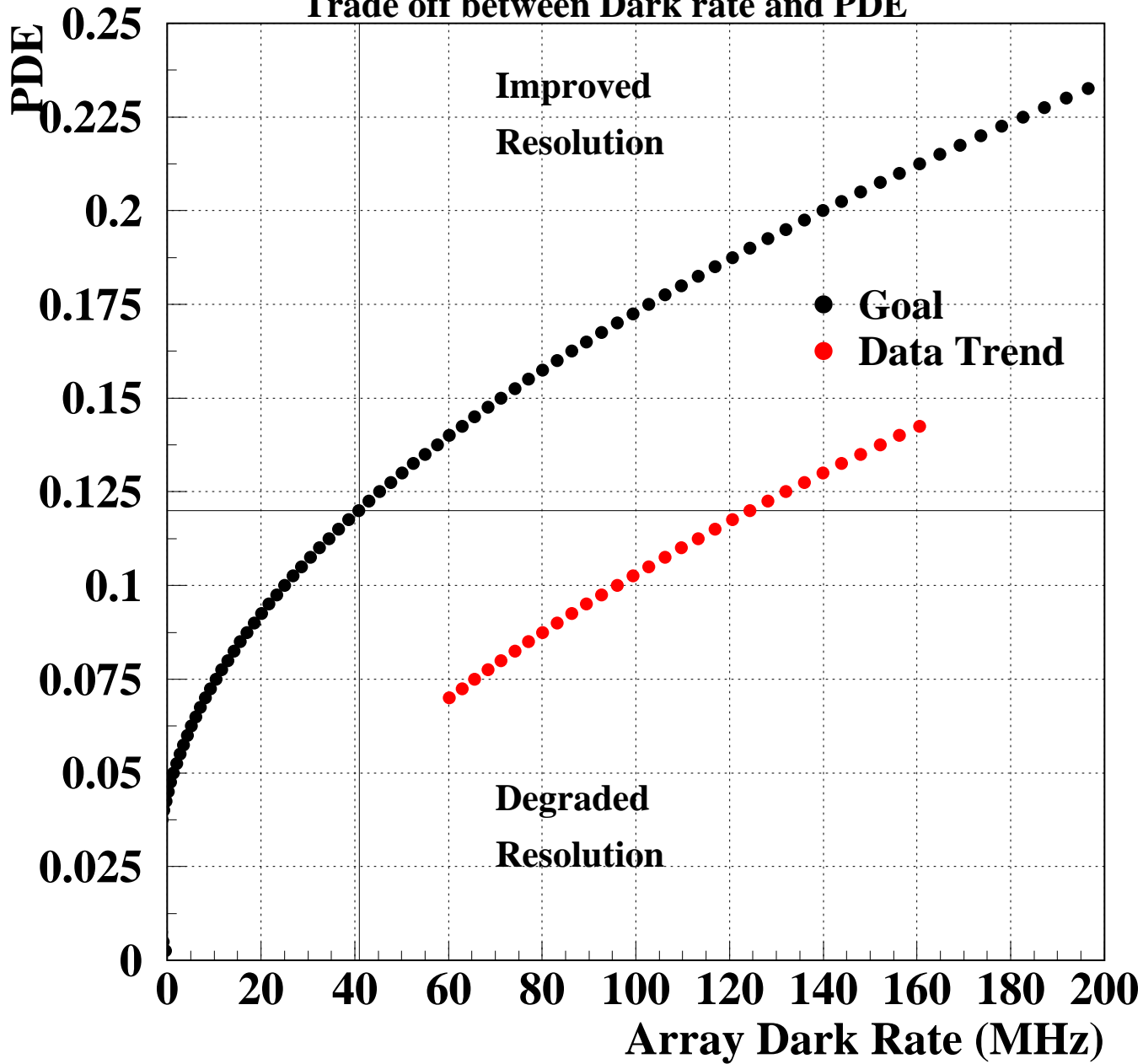
Trade off between Dark rate and PDE
