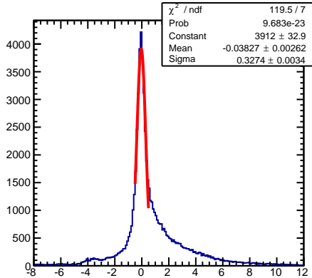
E = 0-0.2 GeV
