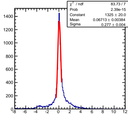
E = 0.4-0.6 GeV
