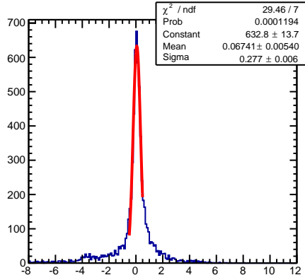
E = 0.6-0.8 GeV
