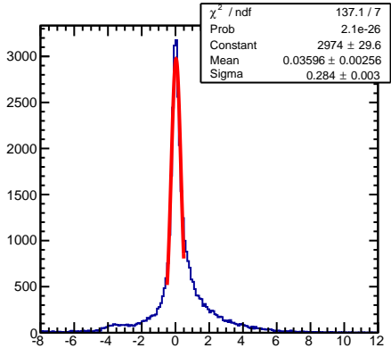
E = 0.2-0.4 GeV
