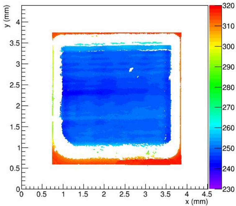
Figure UC30-27-3: Zygo image after 3 passes
