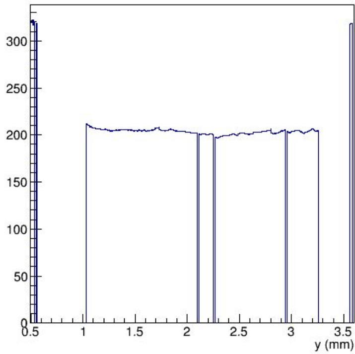
Figure: Cross sectional projection of y axis after pass 6. total cut depth approximately 110 \mu m
