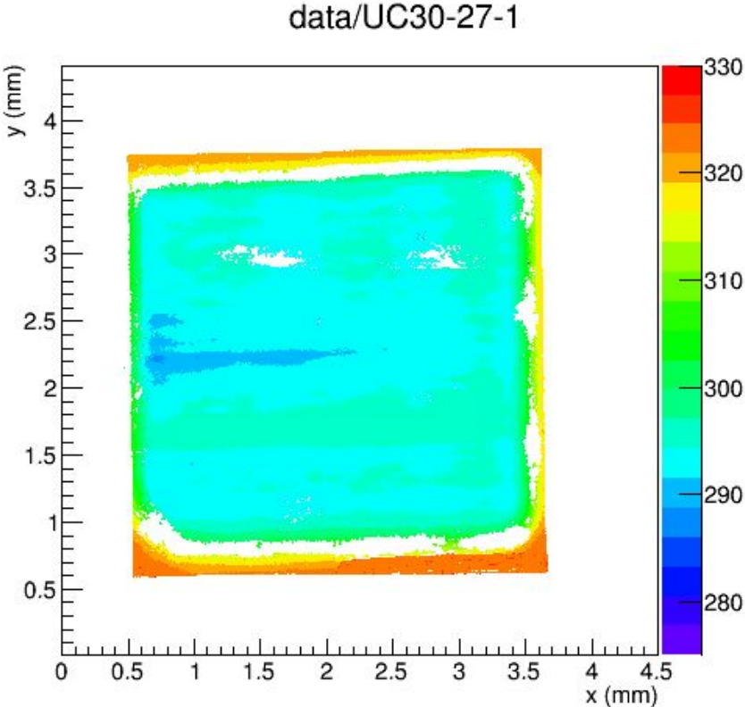
Figure UC30-27-1: Zygo image of sample after one pass of the milling program
