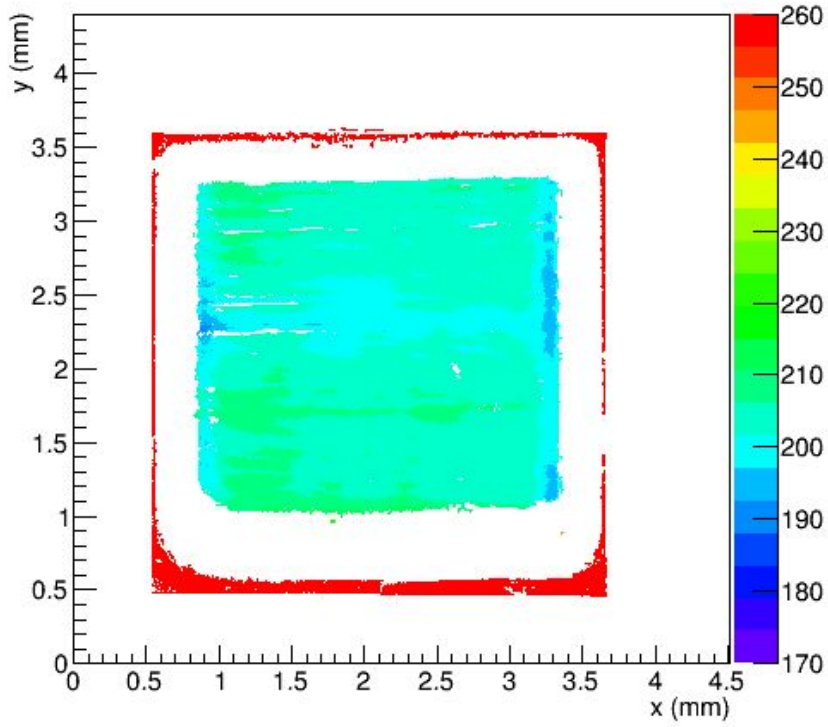
Figure UC30-27-6: Zygo image of sample after 6 passes
