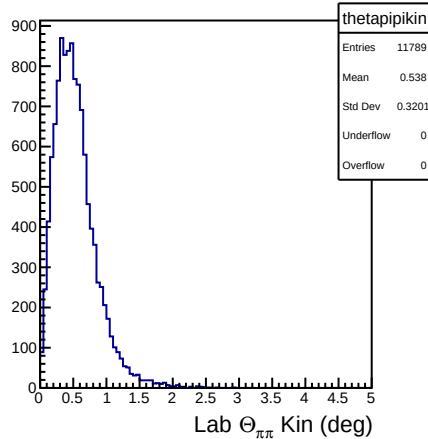
DSelector_Z2pi0_trees_test_flat_100000
