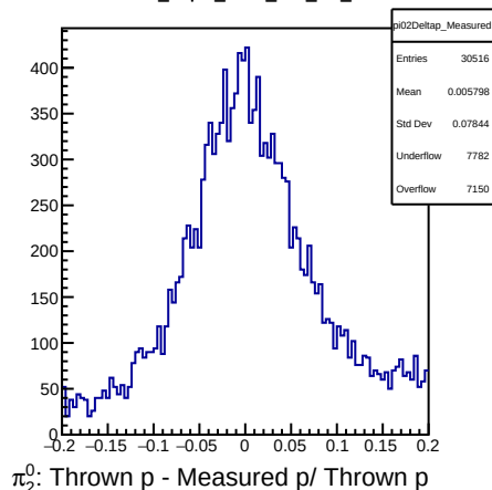
DSelector_Z2pi0_trees_test_flat_100000
