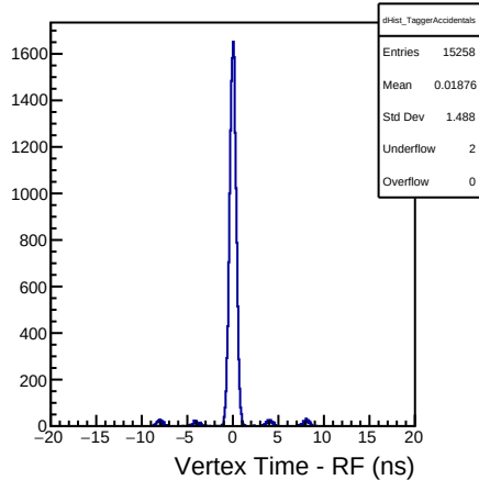
DSelector_Z2pi0_trees_test_flat_100000
