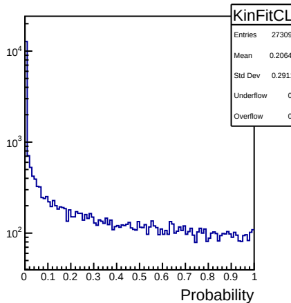
DSelector_Z2pi0_trees_test_flat_100000
