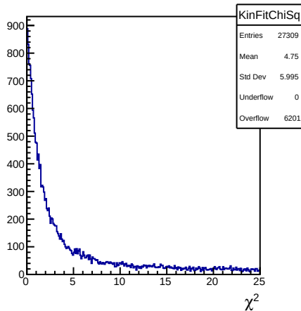
DSelector_Z2pi0_trees_test_flat_100000
