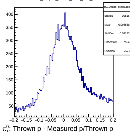
DSelector_Z2pi0_trees_test_flat_100000
