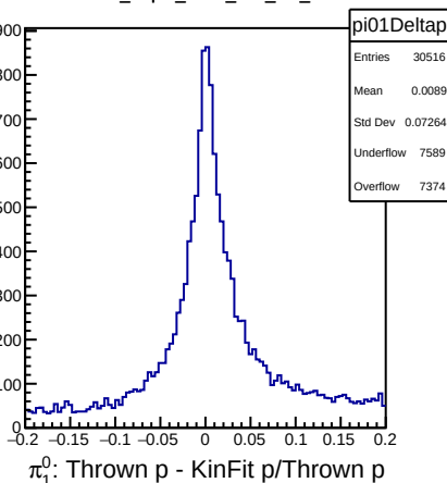
DSelector_Z2pi0_trees_test_flat_100000
