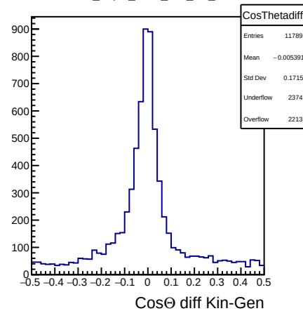
DSelector_Z2pi0_trees_test_flat_100000
