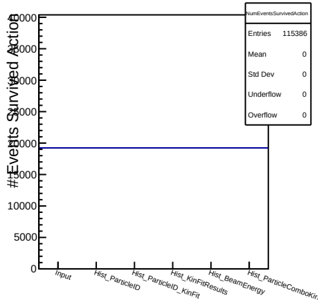
DSelector_Z2pi0_trees_test_flat_100000
