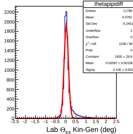
DSelector_Z2pi0_trees_test_flat_100000
