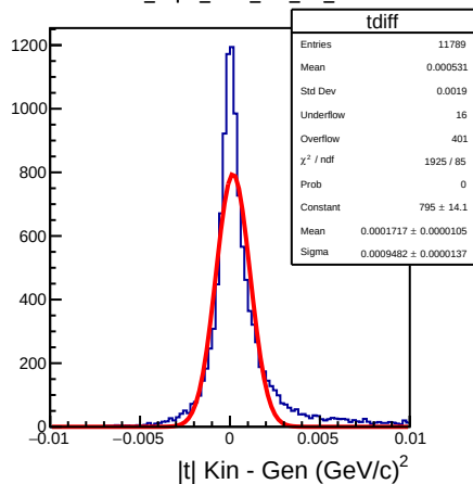
DSelector_Z2pi0_trees_test_flat_100000
