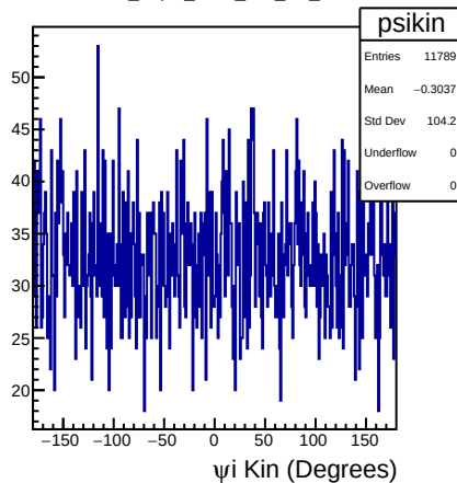
DSelector_Z2pi0_trees_test_flat_100000
