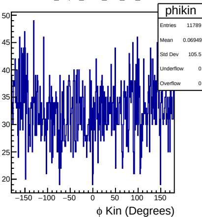
DSelector_Z2pi0_trees_test_flat_100000
