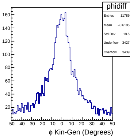
DSelector_Z2pi0_trees_test_flat_100000
