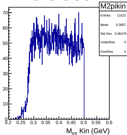
DSelector_Z2pi0_trees_test_flat_100000
