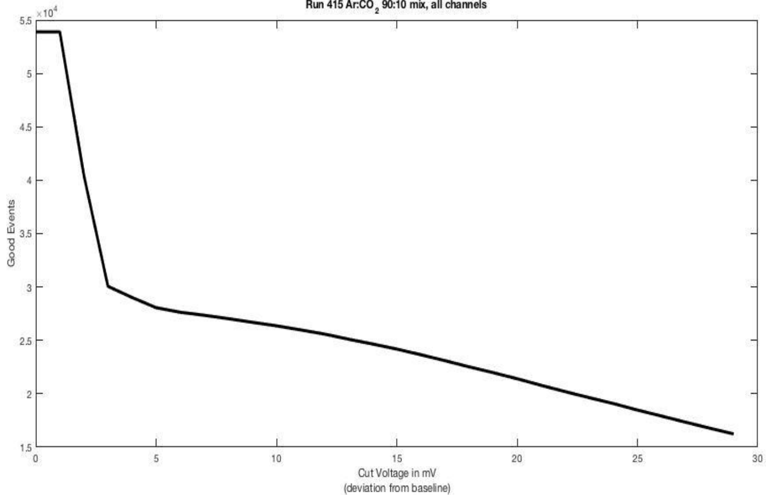
Run 415 Ar:CO 2 90:10 mix, all channels
