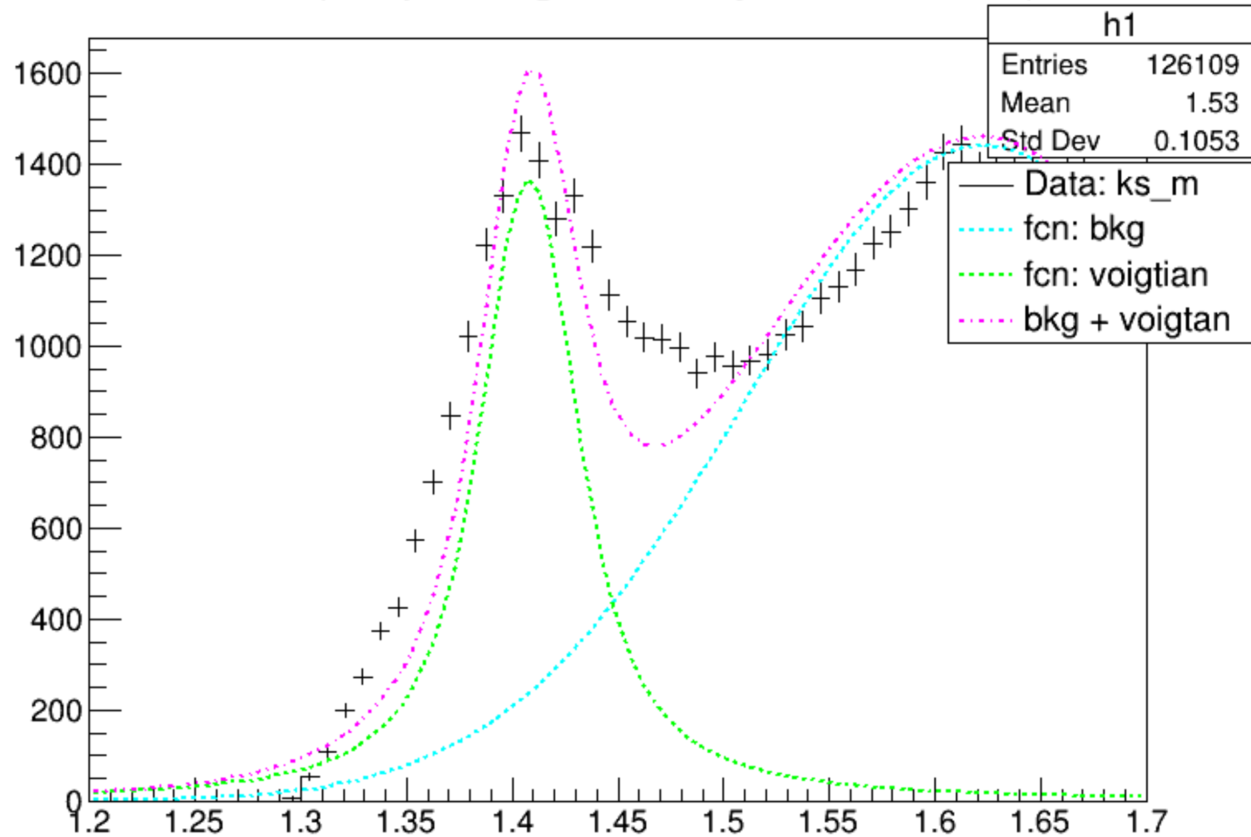
f1_m (keep charged K*, reject neutral K*)
