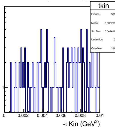
DSelector_Z2pi0_trees_bggen
