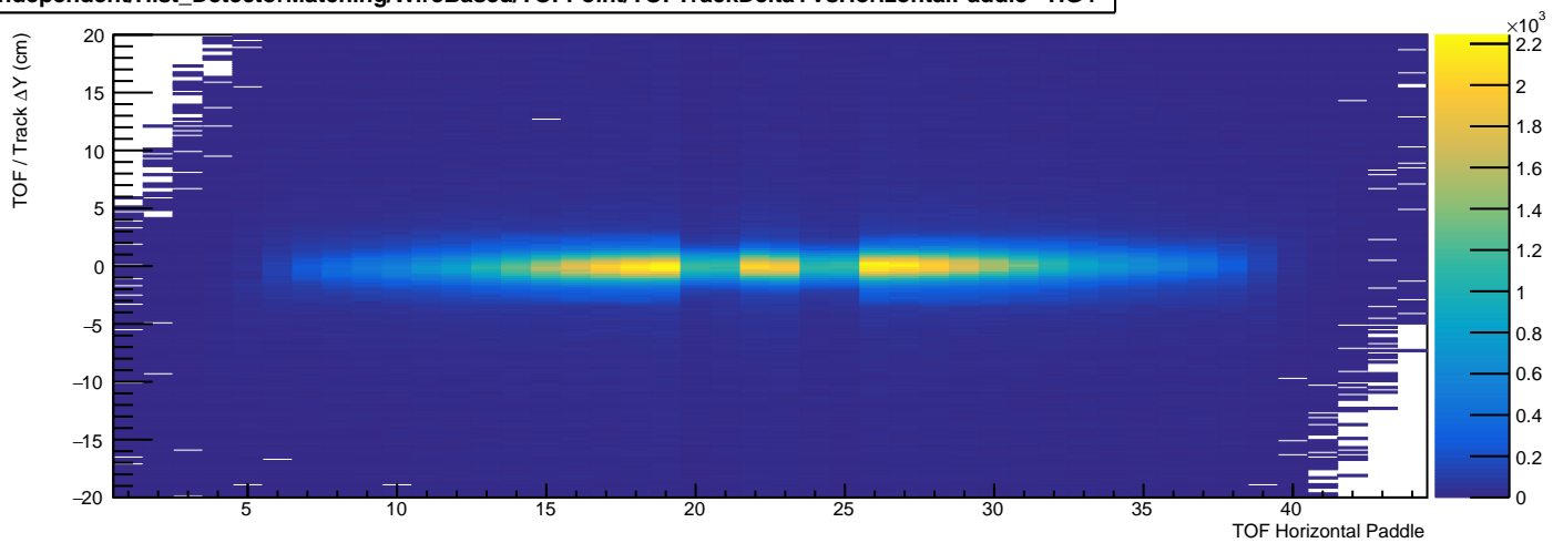
/Independent/Hist_DetectorMatching/WireBased/TOFPoint/TOFTrackDeltaYVsHorizontalPaddle - HG4
