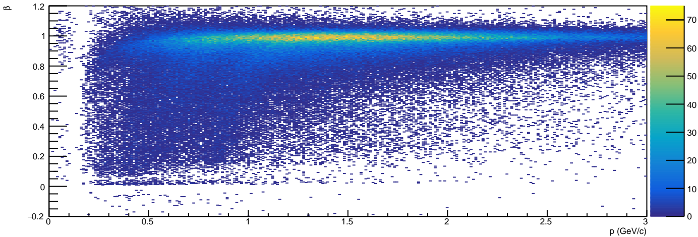
/Independent/Hist_DetectorPID/BCAL/BetaVsP_q - HG4
