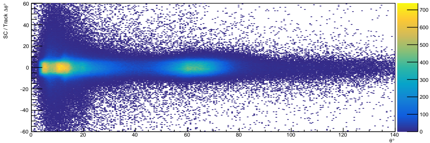
/Independent/Hist_DetectorMatching/WireBased/SC/SCTrackDeltaPhiVsTheta - HG4
