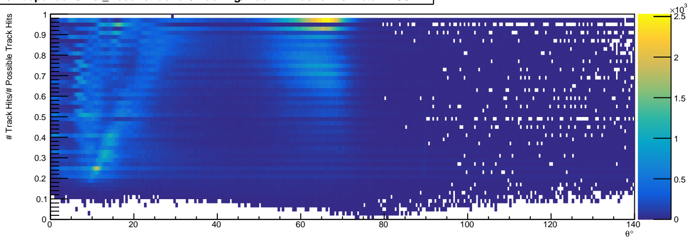
/Independent/Hist_Reconstruction/Tracking/TrackHitFractionVsTheta - HG3
