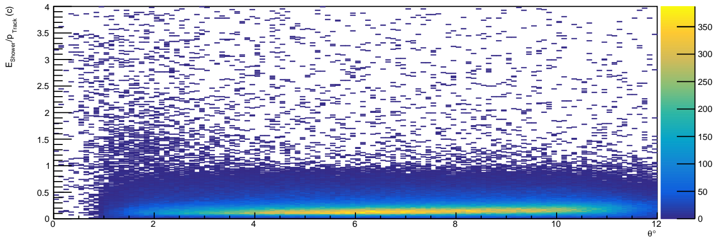
/Independent/Hist_DetectorPID/FCAL/EOverPVsTheta_q- - HG3
