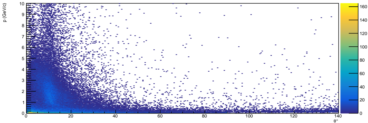
/Independent/Hist_Reconstruction/Tracking/q-/PVsTheta_TimeBased_LowTrackFOM_q- - HG3
