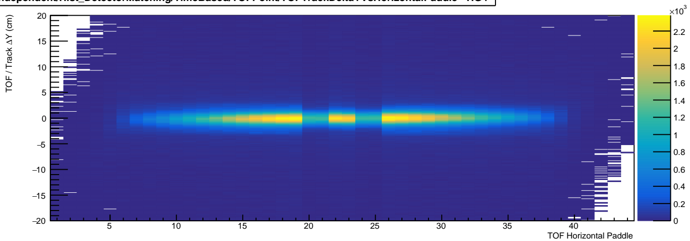
/Independent/Hist_DetectorMatching/TimeBased/TOFPoint/TOFTrackDeltaYVsHorizontalPaddle - HG4
