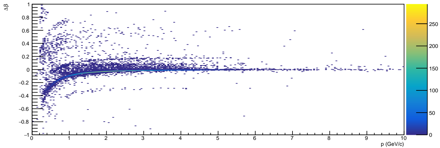
/Independent/Hist_DetectorPID/TOF/DeltaBetaVsP_K- - HG4
