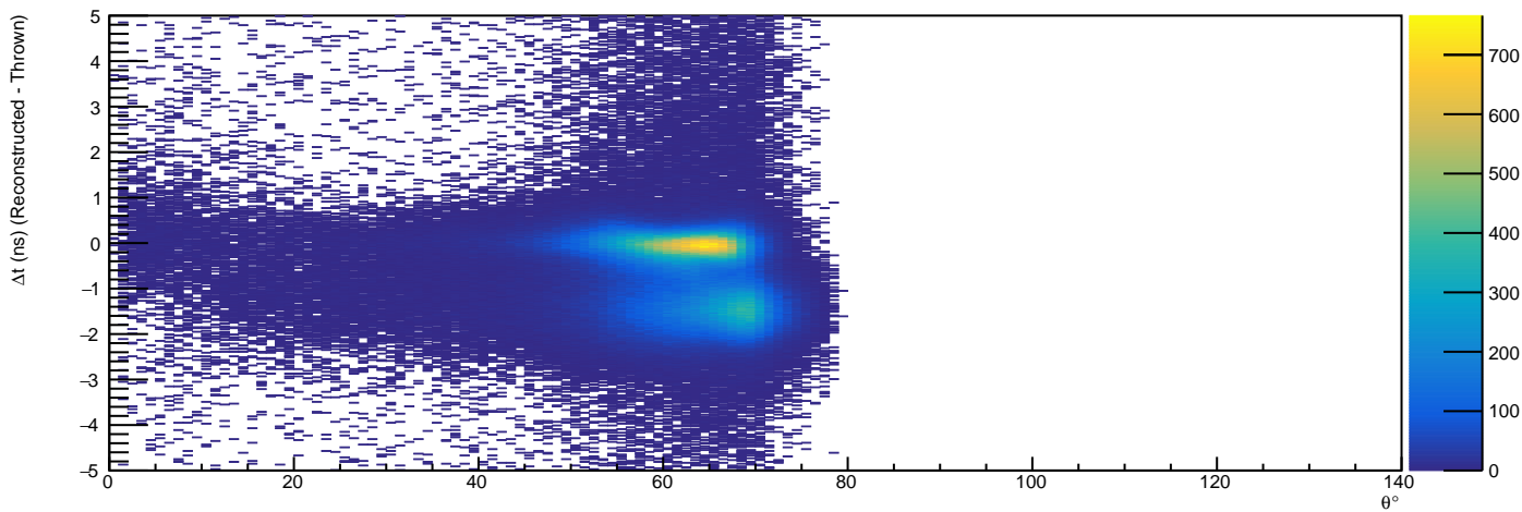
/Independent/Hist_GenReconTrackComparison/Proton/DeltaTVsTheta - HG4
