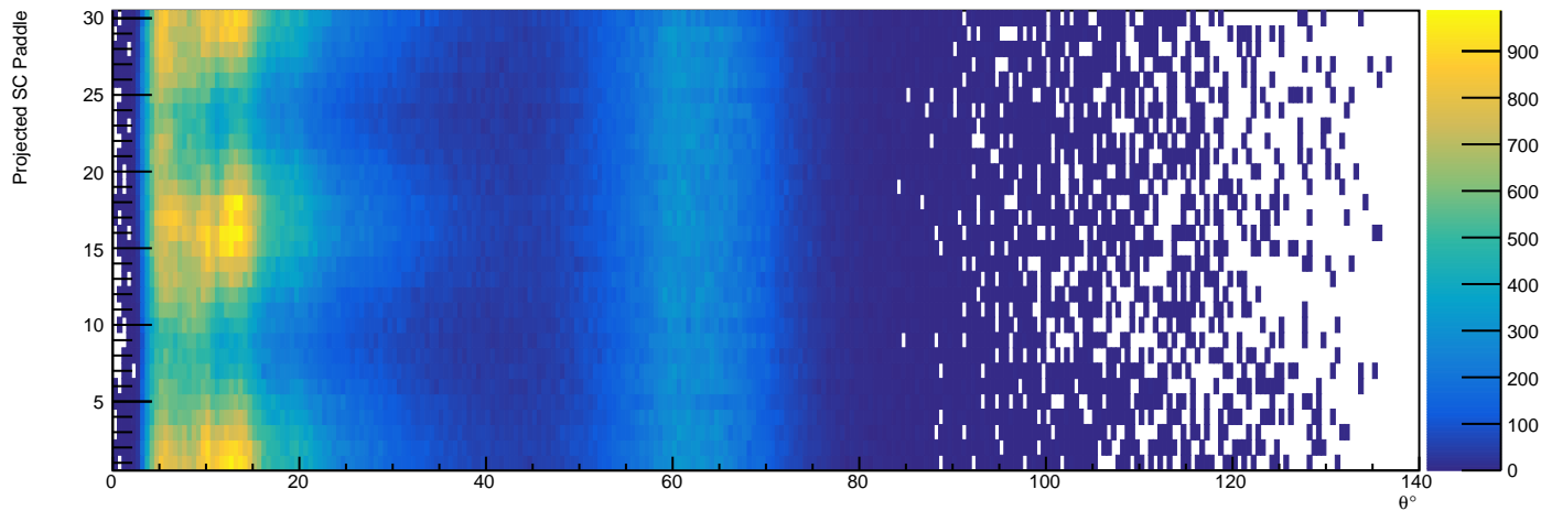
/Independent/Hist_DetectorMatching/WireBased/SC/SCPaddleVsTheta_HasHit - HG4
