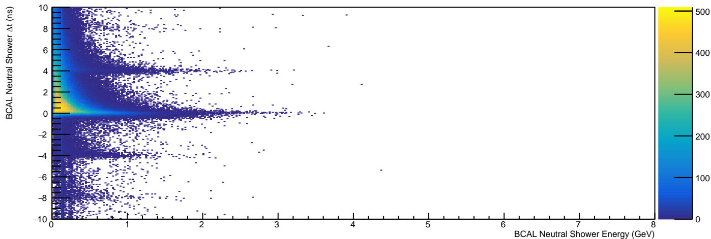
/Independent/Hist_Neutrals/BCALNeutralShowerDeltaTVsE - HG4
