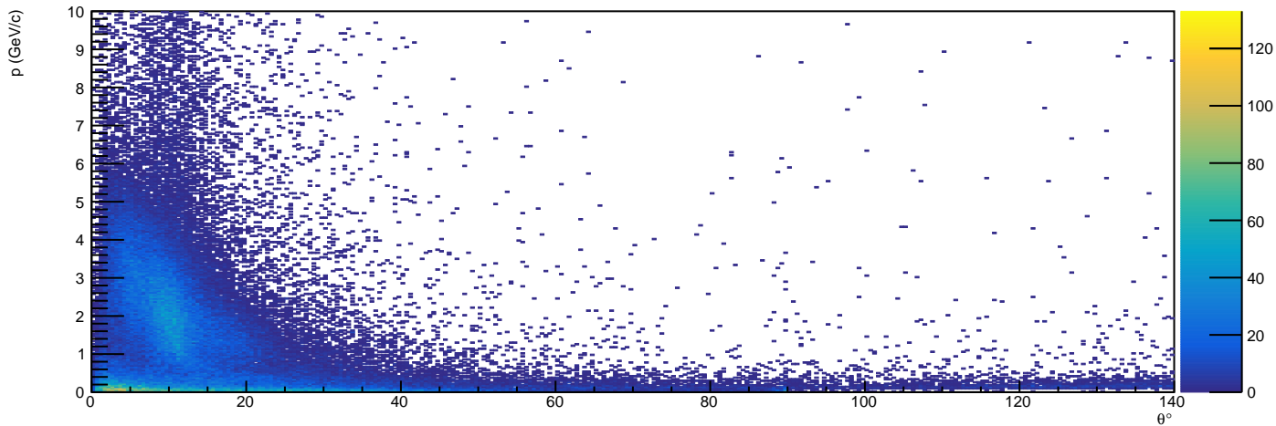
/Independent/Hist_Reconstruction/Tracking/q-/PVsTheta_TimeBased_LowTrackFOM_q- - HG4
