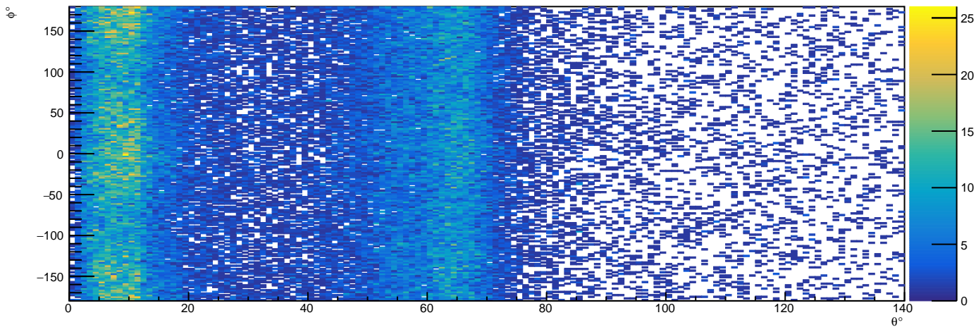
/Independent/Hist_DetectedParticleKinematics/Proton/PhiVsTheta - HG4
