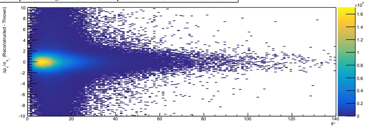
/Independent/Hist_GenReconTrackComparison/Pi+/Pulls/PxPullIVsTheta - HG3
