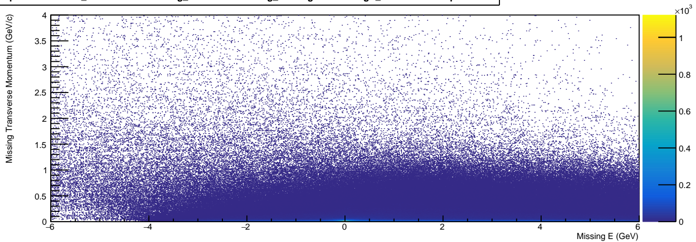
/Independent/Combo_Construction/Missing_Mass/NoneMissing_MissingPtVsMissingE_PreMissMassSqCut - HG4
