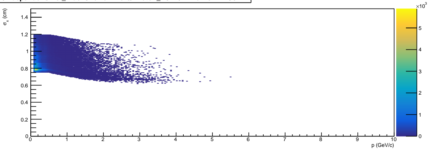
/Independent/Hist_TrackShowerErrors/Photon_FCAL/XErrorVsP - HG3
