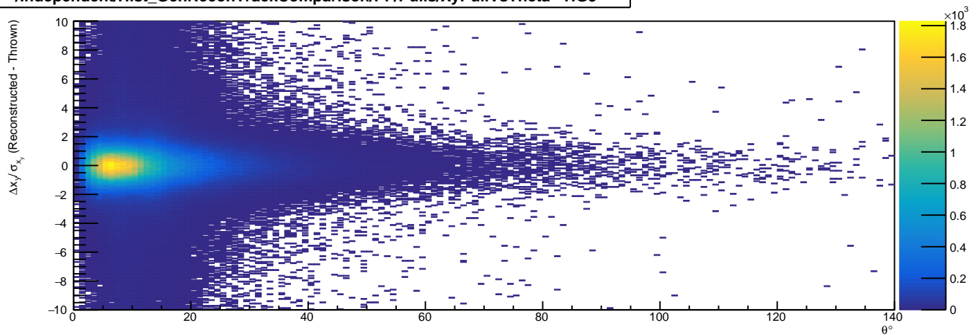
/Independent/Hist_GenReconTrackComparison/Pi-/Pulls/XyPullIVsTheta - HG3
