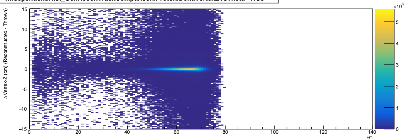
/Independent/Hist_GenReconTrackComparison/Proton/DeltaVertexZVsTheta - HG3
