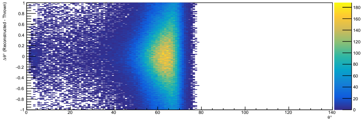
/Independent/Hist_GenReconTrackComparison/Proton/DeltaThetaVsTheta - HG3
