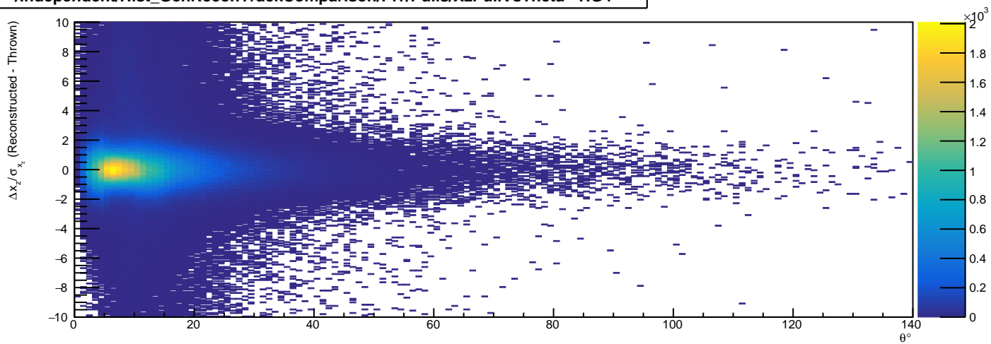
/Independent/Hist_GenReconTrackComparison/Pi+/Pulls/XzPullVsTheta - HG4
