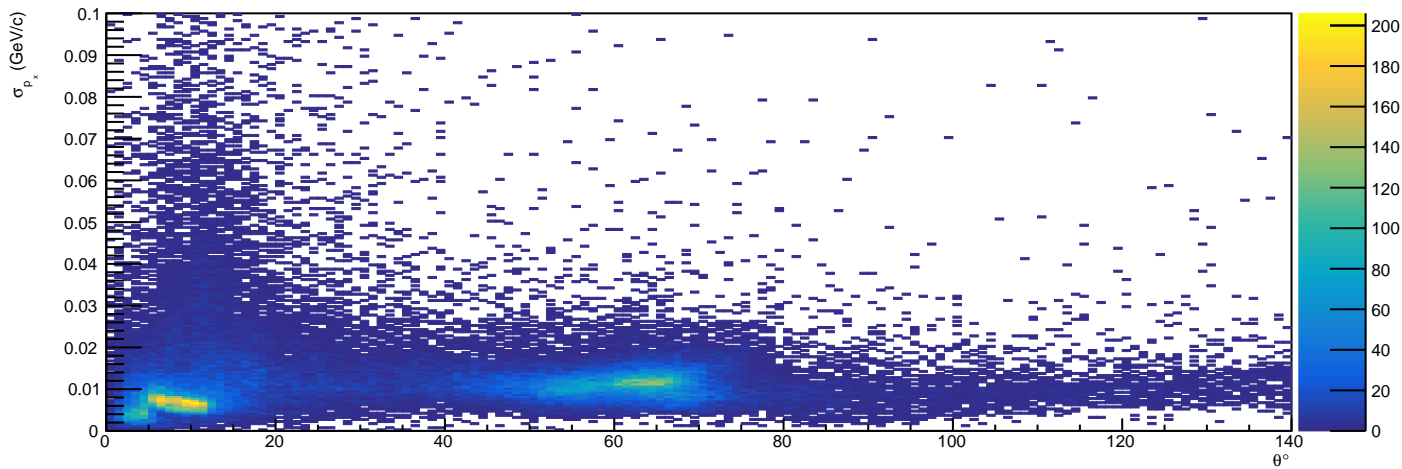
/Independent/Hist_TrackShowerErrors/Proton/PxErrorVsTheta - HG4
