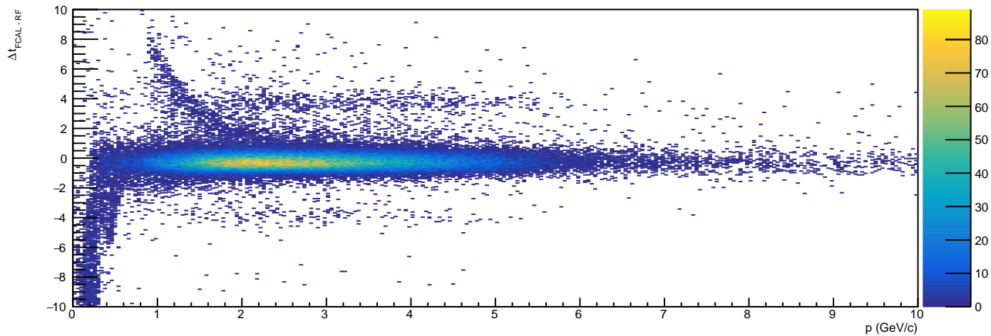
/Independent/Hist_DetectorPID/FCAL/DeltaTVsP_Pi+ - HG4
