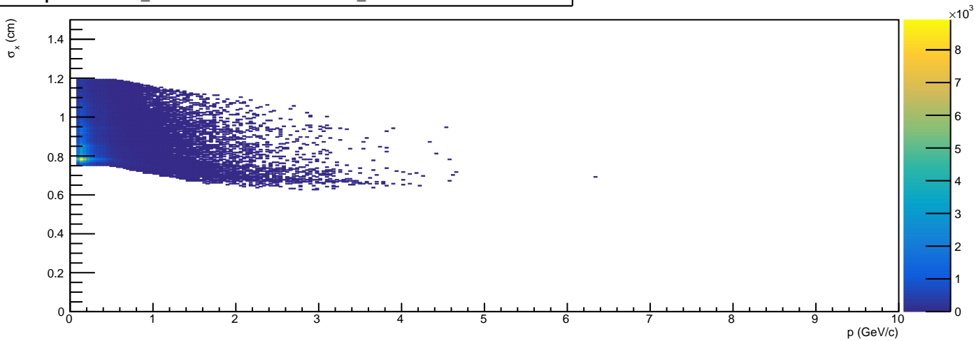
/Independent/Hist_TrackShowerErrors/Photon_FCAL/XErrorVsP - HG4
