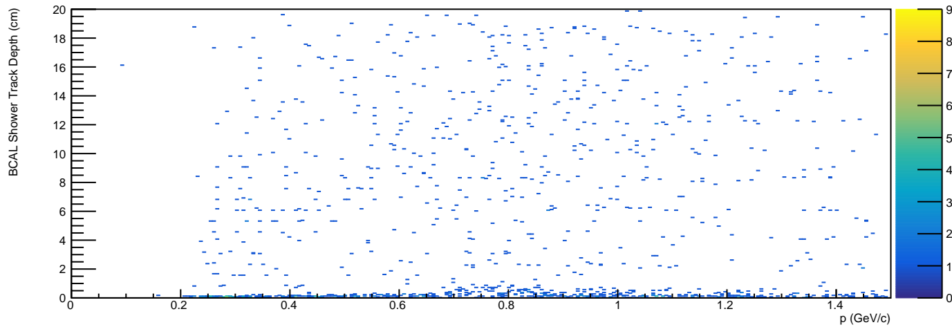
/Independent/Hist_DetectorMatchParams/ReconstructedPID/K+/BCALShowerTrackDepthVsP - HG4
