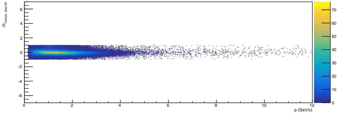
/Independent/Combo_Construction/PID/Pi+/Best_RFDeltaTVsP_BCAL - HG4
