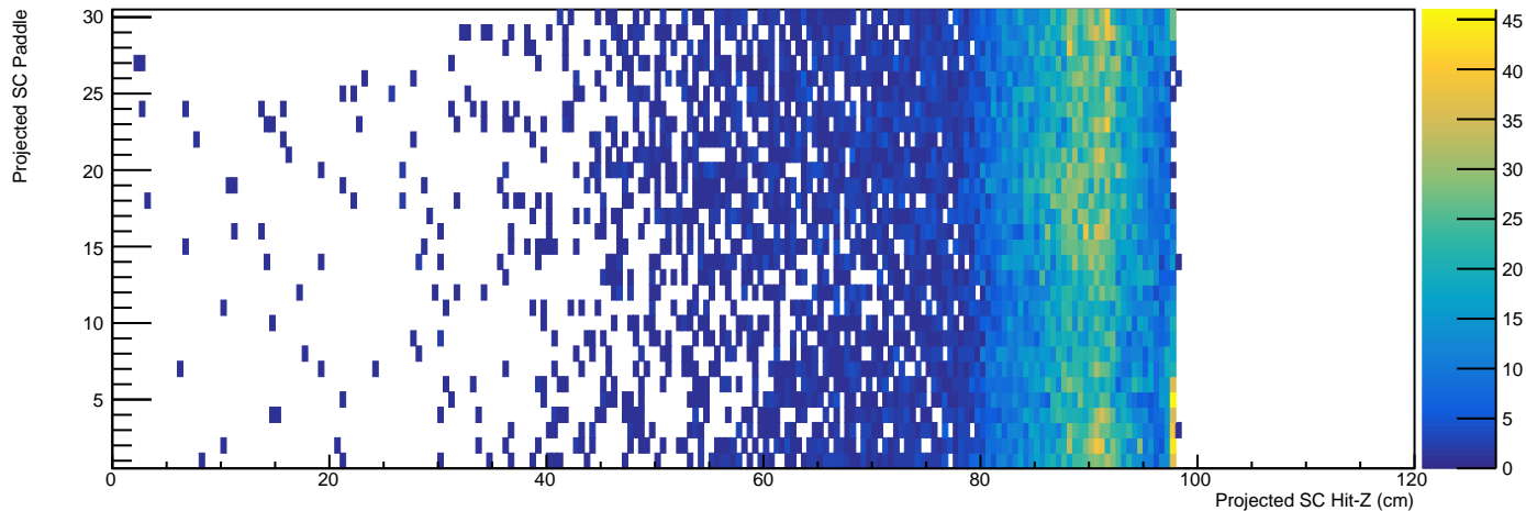
/Independent/Hist_DetectorMatching/TimeBased/SC/SCPaddleVsZ_NoHit - HG4
