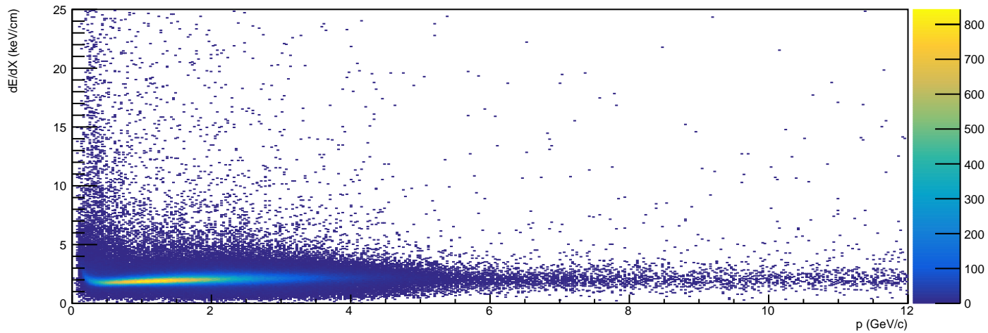
/Independent/Combo_Construction/PID/Pi-/dEdxVsP_CDC - HG4
