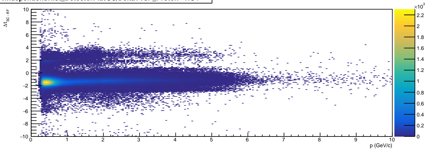
/Independent/Hist_DetectorPID/SC/DeltaTVsP_Proton - HG4
