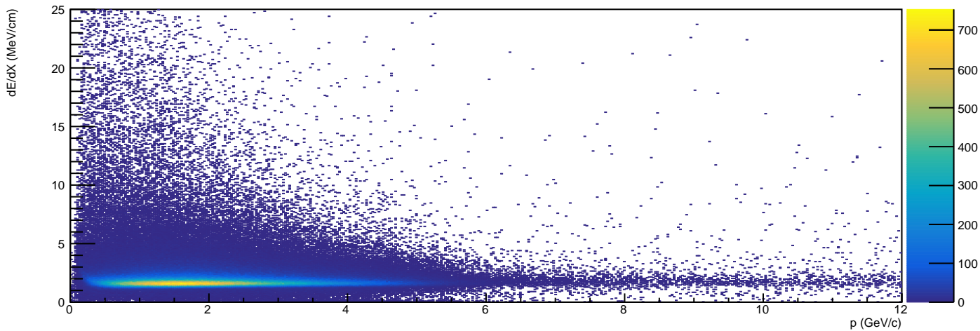
/Independent/Combo_Construction/PID/Pi-dEdxVsP_ST - HG4
