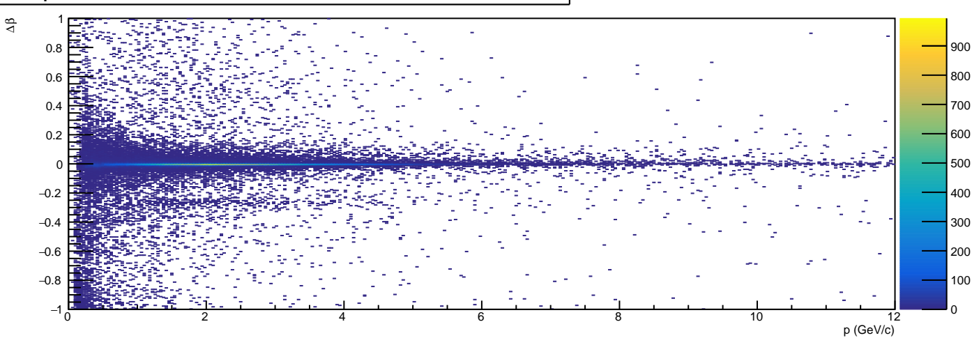
/Independent/Hist_DetectedParticleKinematics/Pi-DeltaBetaVsP - HG4
