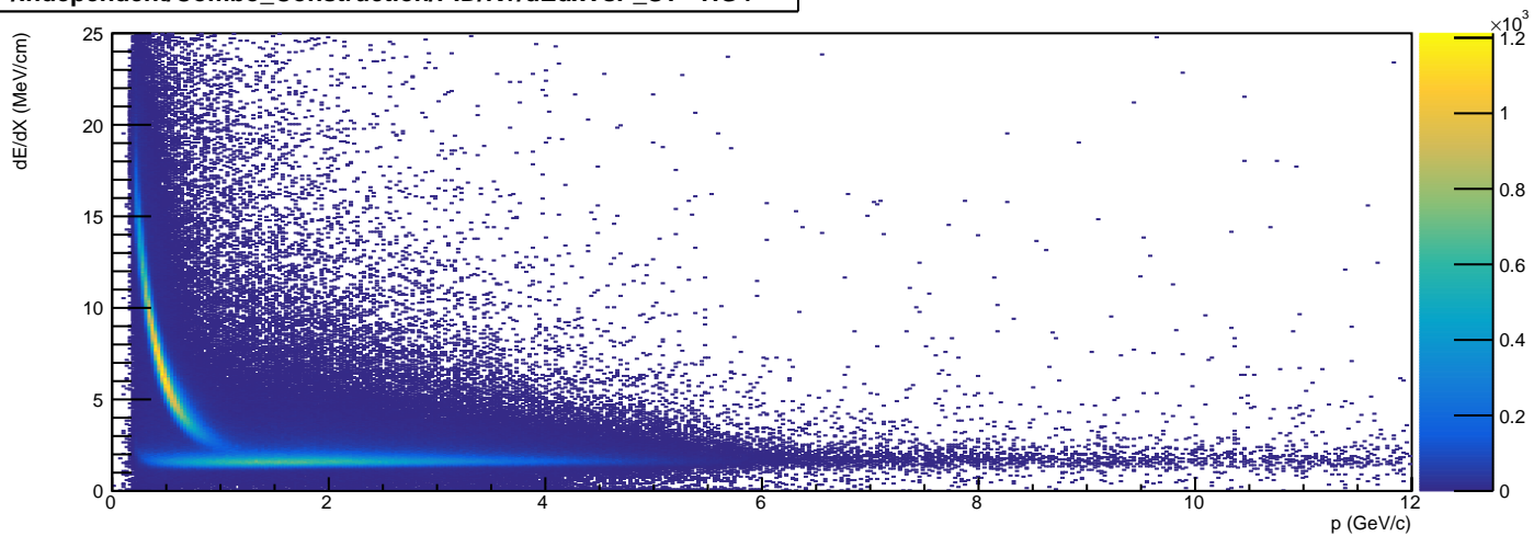
/Independent/Combo_Construction/PID/K+/dEdxVsP_ST - HG4
