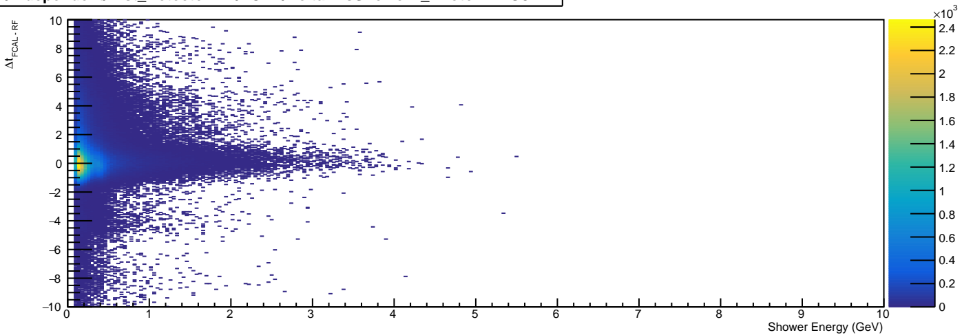
/Independent/Hist_DetectorPID/FCAL/DeltaTVsShowerE_Photon - HG3
