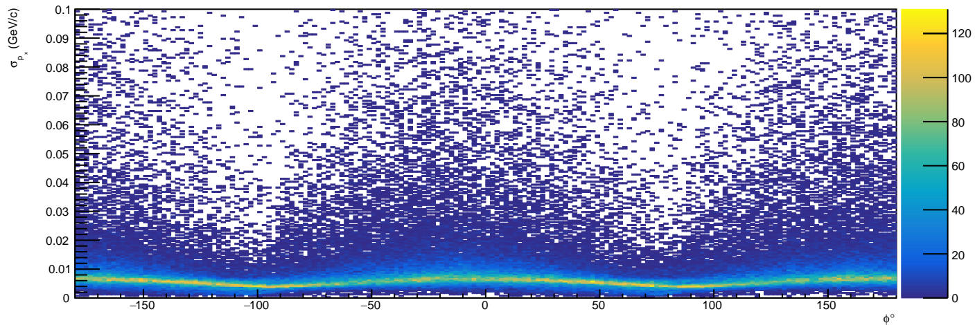
/Independent/Hist_TrackShowerErrors/Pi-PxErroVsPhi - HG4
