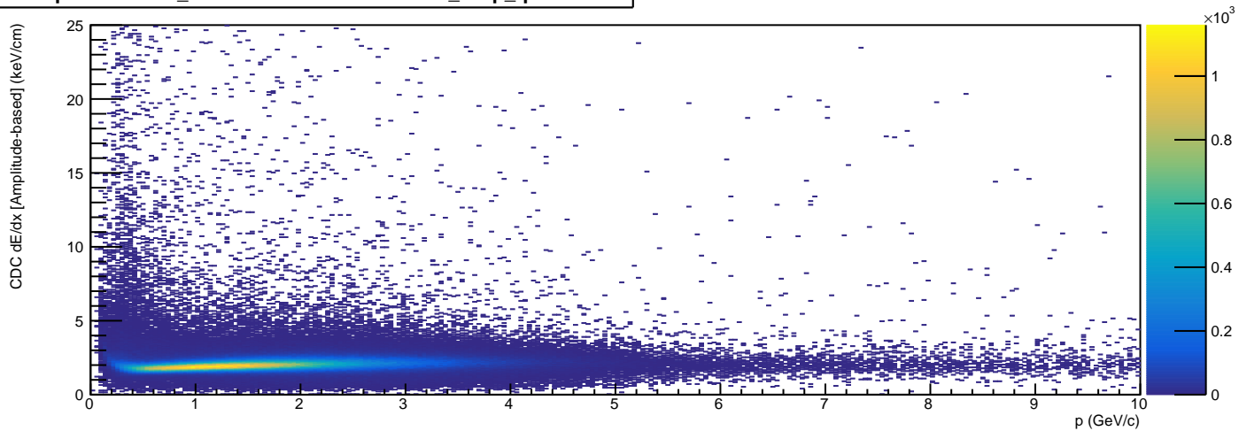
/Independent/Hist_DetectorPID/CDC/dEdXVsP_Amp_q - HG4
