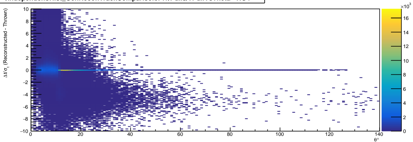
/Independent/Hist_GenReconTrackComparison/Pi+/Pulls/TPullVsTheta - HG4
