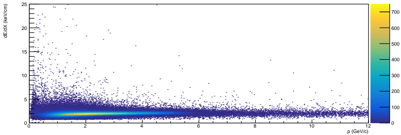
/Independent/Combo_Construction/PID/K-dEdxVsP_FDC - HG4
