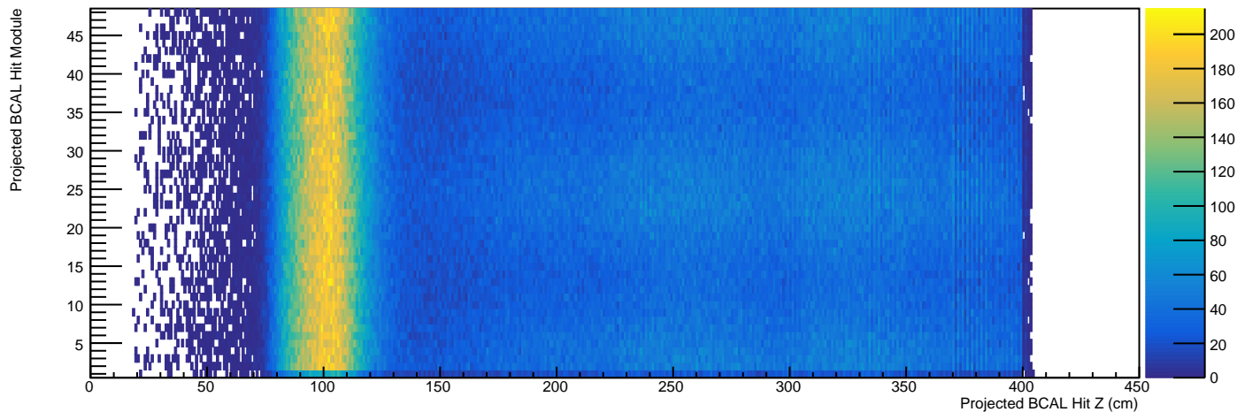
/Independent/Hist_DetectorMatching/TimeBased/BCAL/TrackBCALModuleVsZ_HasHit - HG4
