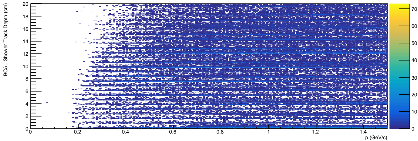
/Independent/Hist_DetectorMatchParams/TruePID/Pi+/BCALShowerTrackDepthVsP - HG4
