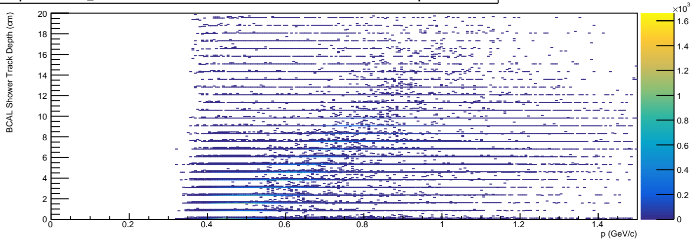
/Independent/Hist_DetectorMatchParams/TruePID/Proton/BCALShowerTrackDepthVsP - HG3
