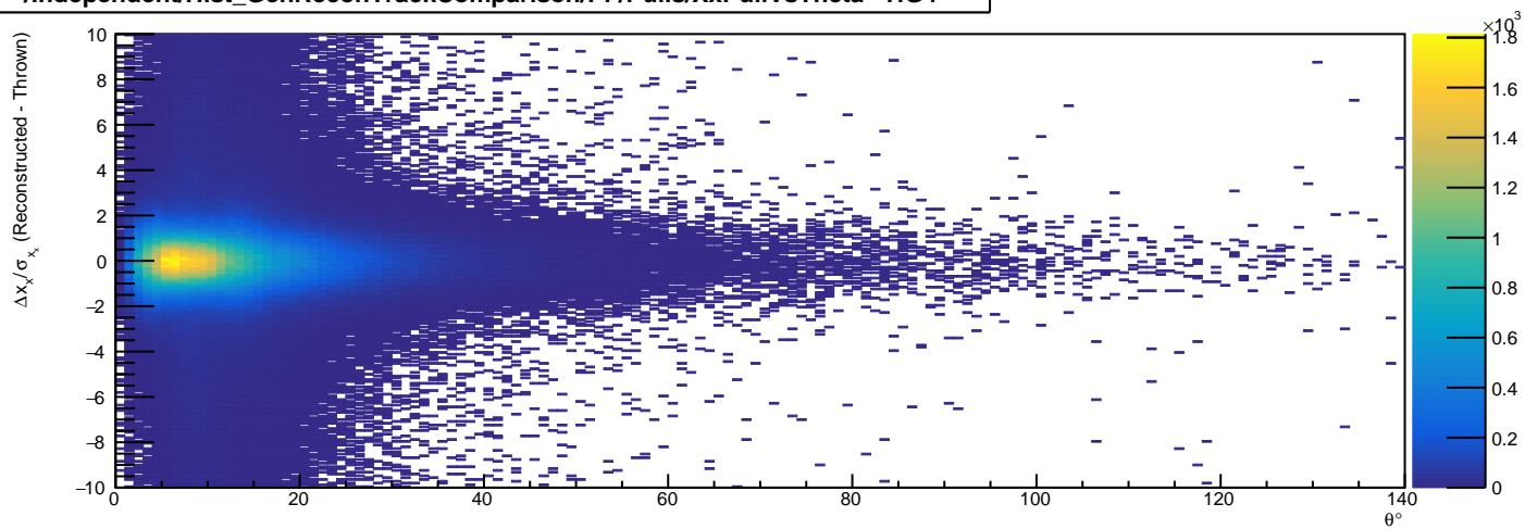
/Independent/Hist_GenReconTrackComparison/Pi-/Pulls/XxPullIVsTheta - HG4
