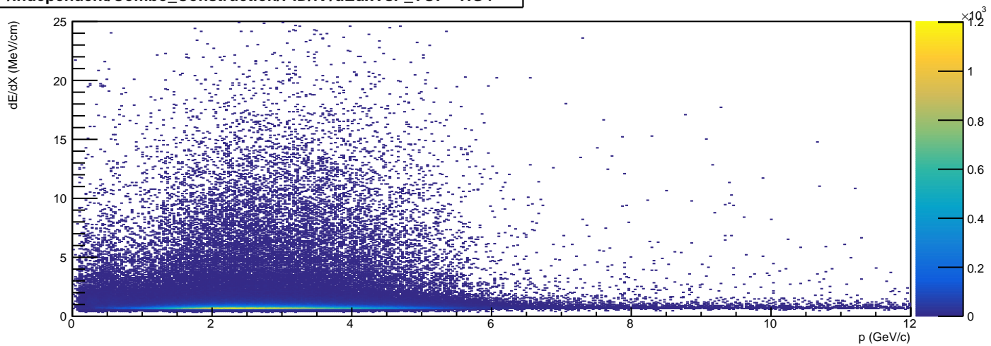
/Independent/Combo_Construction/PID/K-dEdxVsP_TOF - HG4
