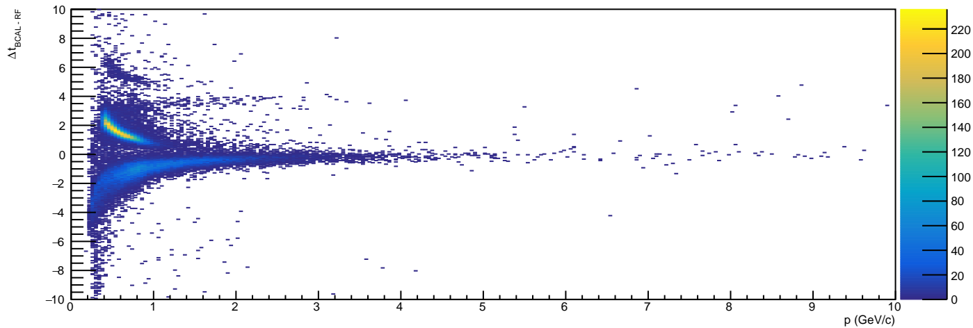
/Independent/Hist_DetectorPID/BCAL/DeltaTVsP_K+ - HG4
