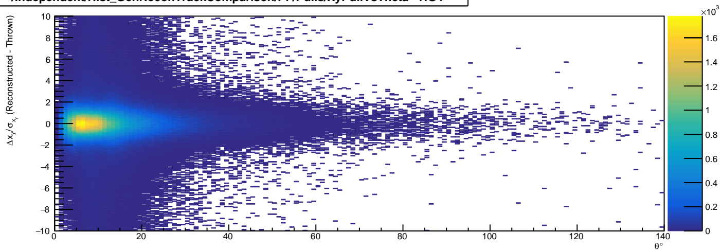
/Independent/Hist_GenReconTrackComparison/Pi-/Pulls/XyPullIVsTheta - HG4
