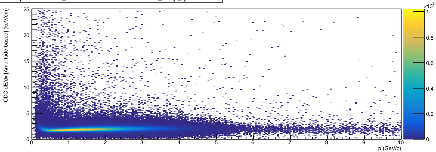
/Independent/Hist_DetectorPID/CDC/dEdXVsP_Amp_q - HG3
