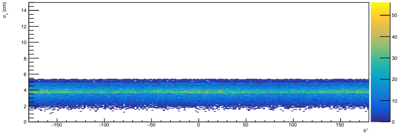
/Independent/Hist_TrackShowerErrors/Photon_BCAL/ZErrorVsPhi - HG4
