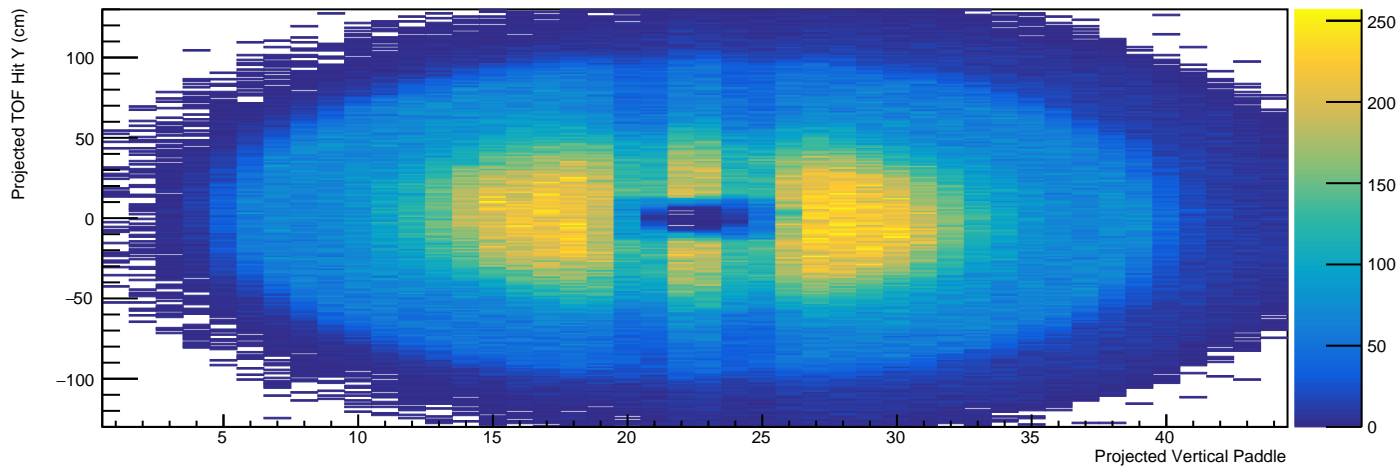
/Independent/Hist_DetectorMatching/WireBased/TOFPaddle/TrackYVsVerticalPaddle_HasHit - HG4
