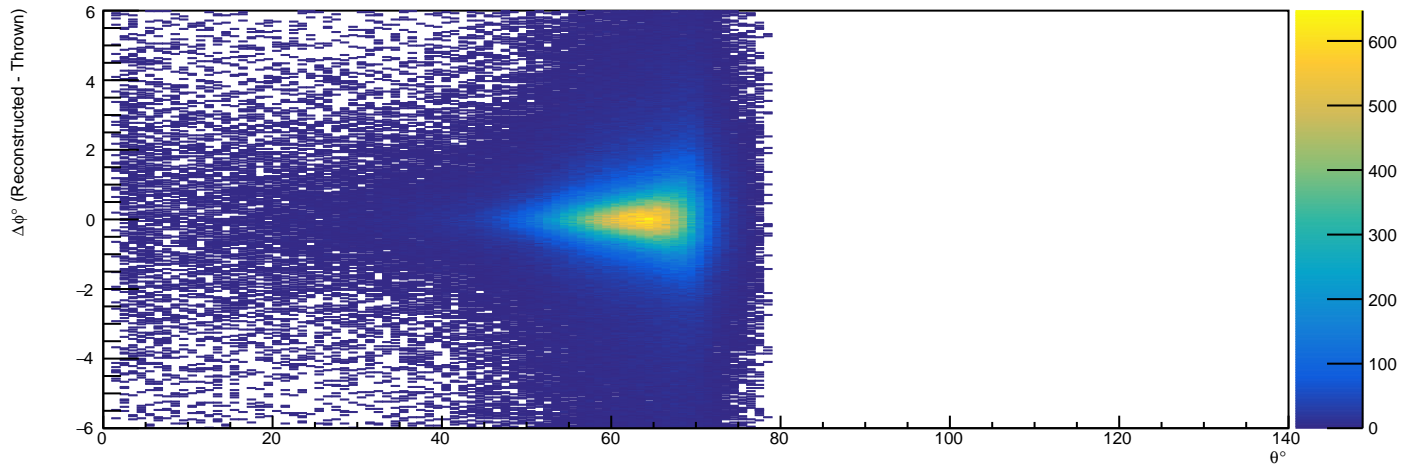
/Independent/Hist_GenReconTrackComparison/Proton/DeltaPhiVsTheta - HG4
