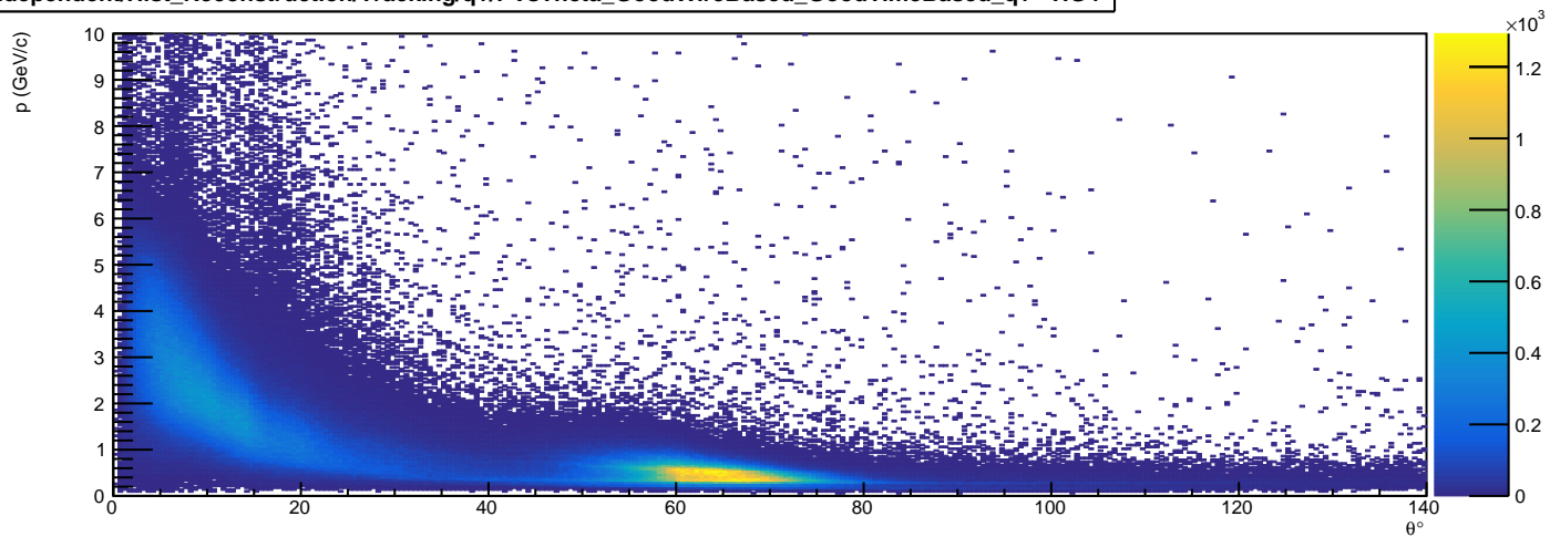
/Independent/Hist_Reconstruction/Tracking/q+/PVsTheta_GoodWireBased_GoodTimeBased_q+ - HG4
