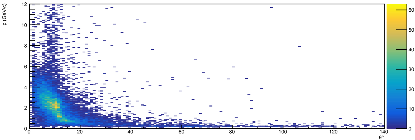
/Independent/Hist_DetectedParticleKinematics/K+/PVsTheta - HG4
