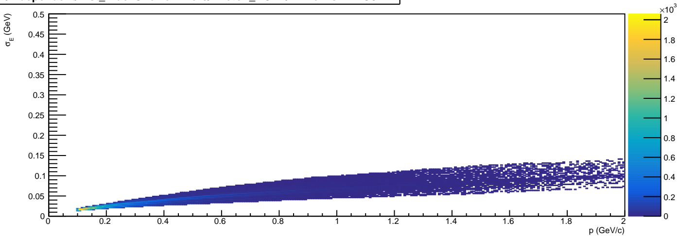
/Independent/Hist_TrackShowerErrors/Photon_BCAL/EErrorVsP - HG3
