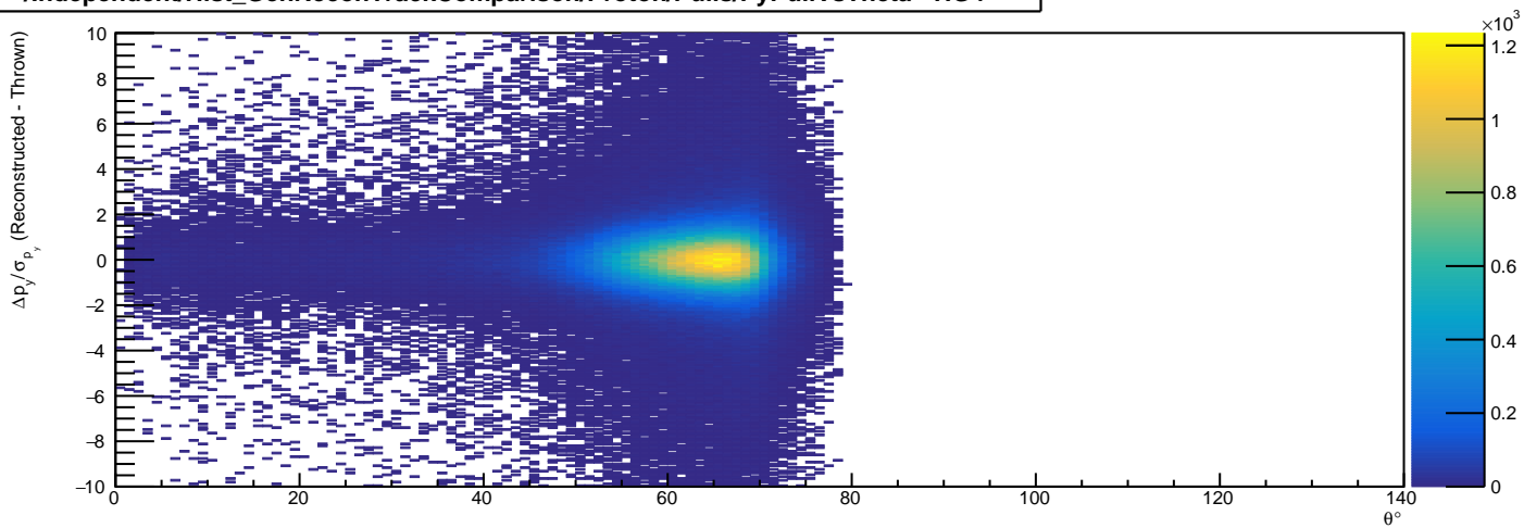
/Independent/Hist_GenReconTrackComparison/Proton/Pulls/PyPullVsTheta - HG4
