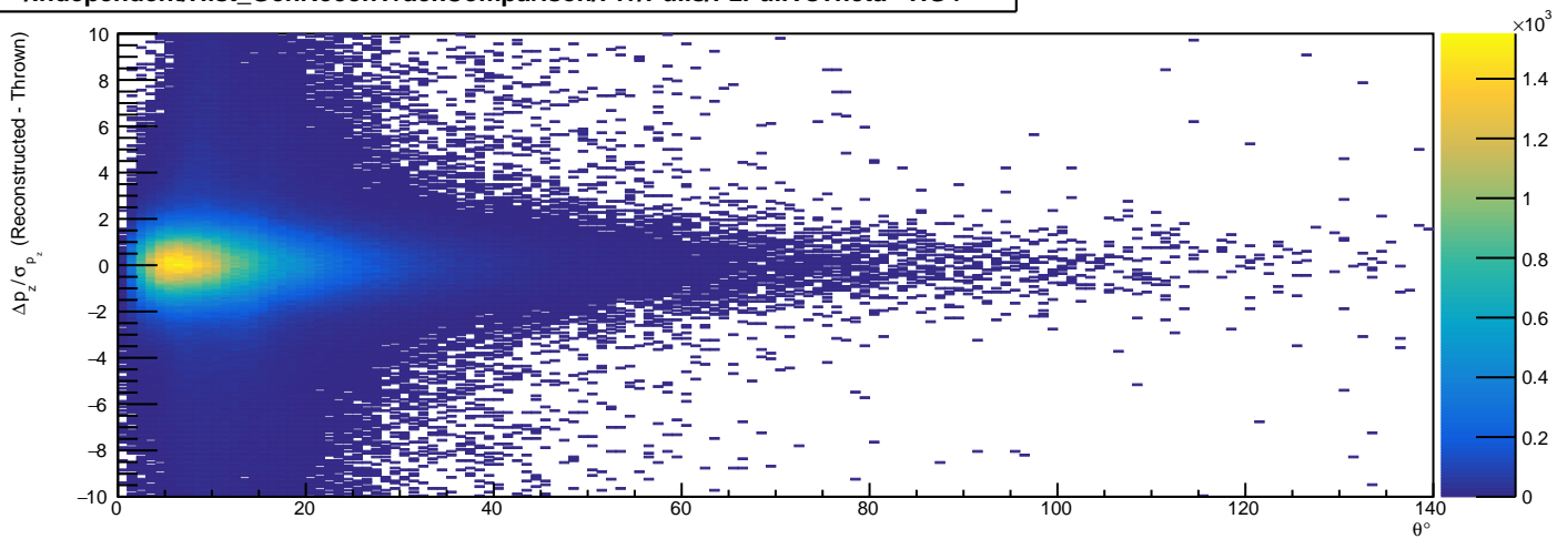
/Independent/Hist_GenReconTrackComparison/Pi+/Pulls/PzPullIVsTheta - HG4
