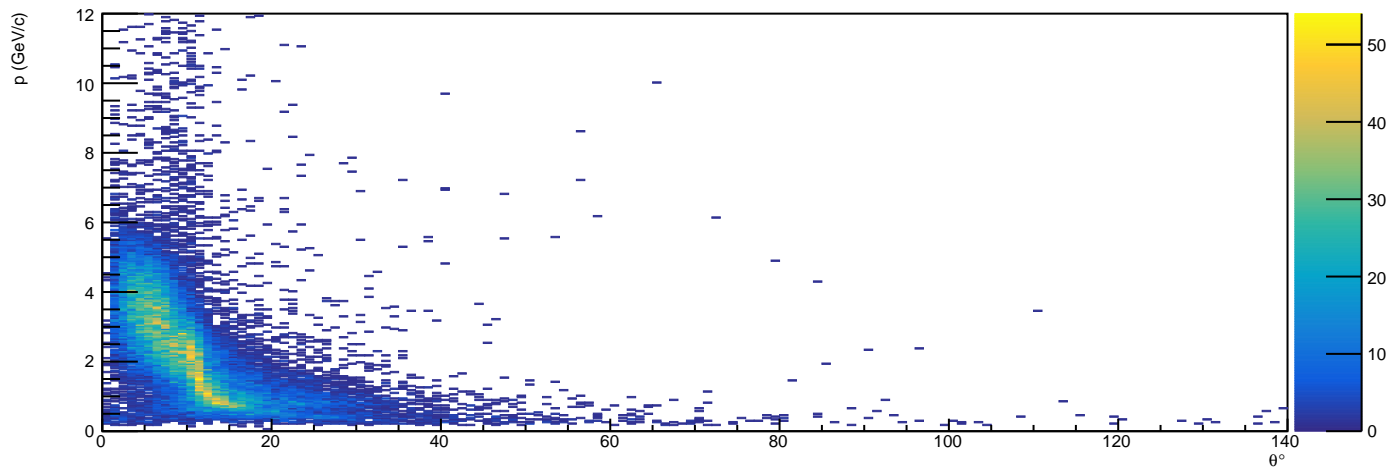
/Independent/Hist_DetectedParticleKinematics/K-/PVsTheta - HG4
