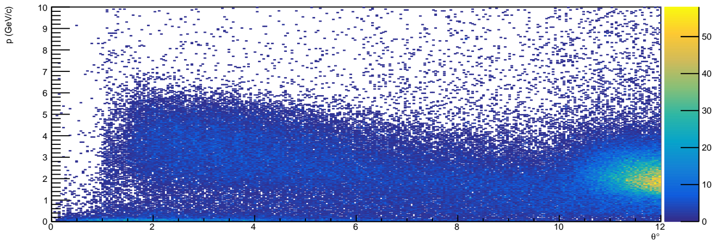
/Independent/Hist_DetectorMatching/TimeBased/FCAL/PVsTheta_NoHit - HG3
