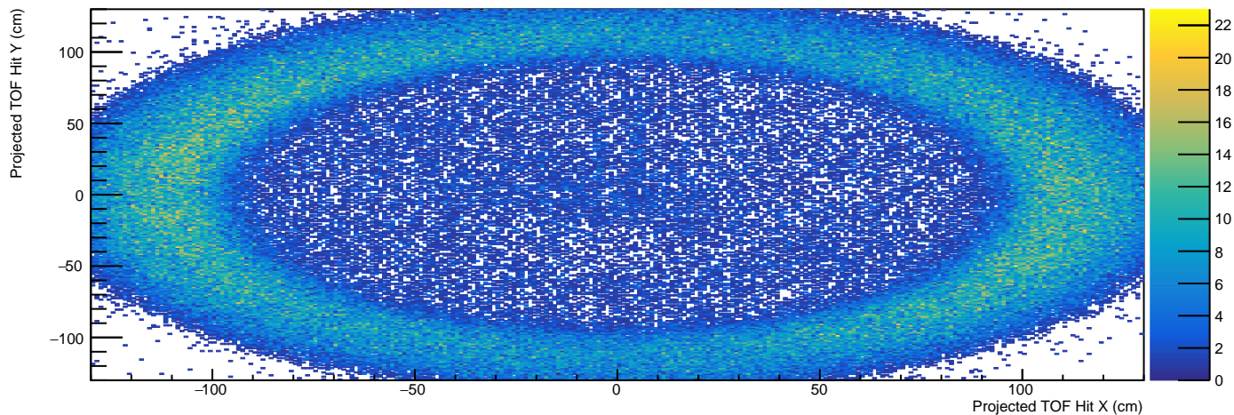
/Independent/Hist_DetectorMatching/WireBased/TOFPoint/TrackTOFYVsX_NoHit - HG4
