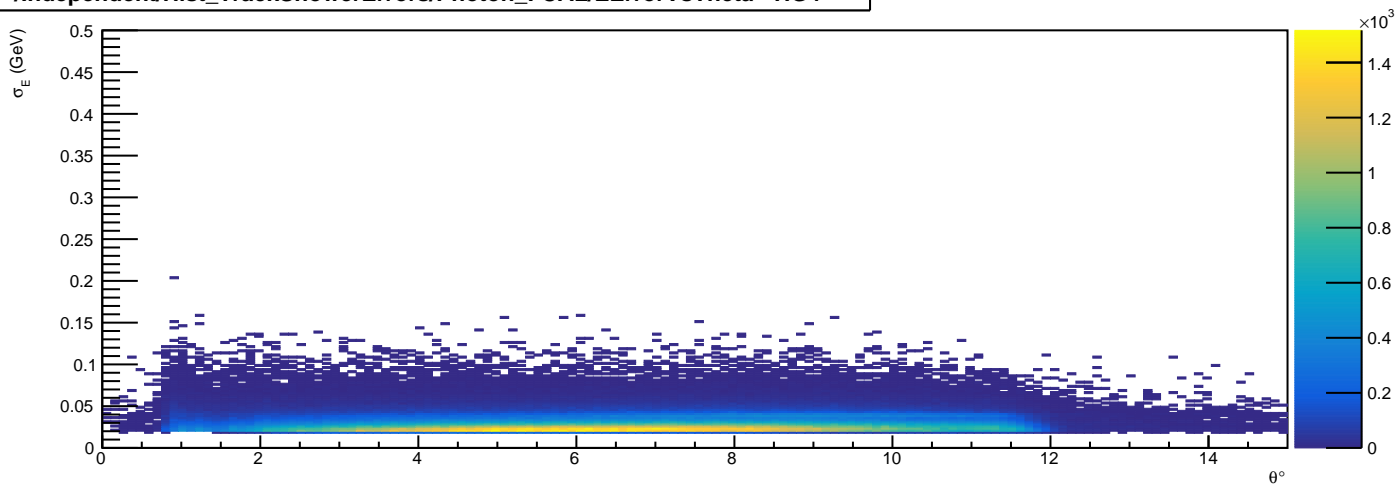
/Independent/Hist_TrackShowerErrors/Photon_FCAL/EErrorVsTheta - HG4
