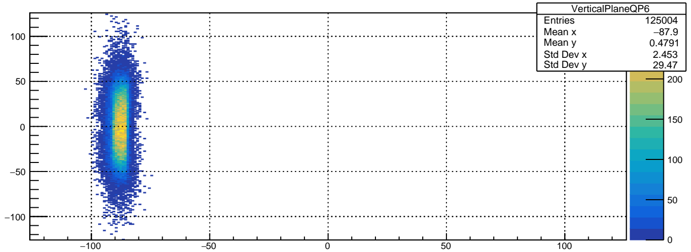
Vertical Plane Paddle 7 Q=+1
