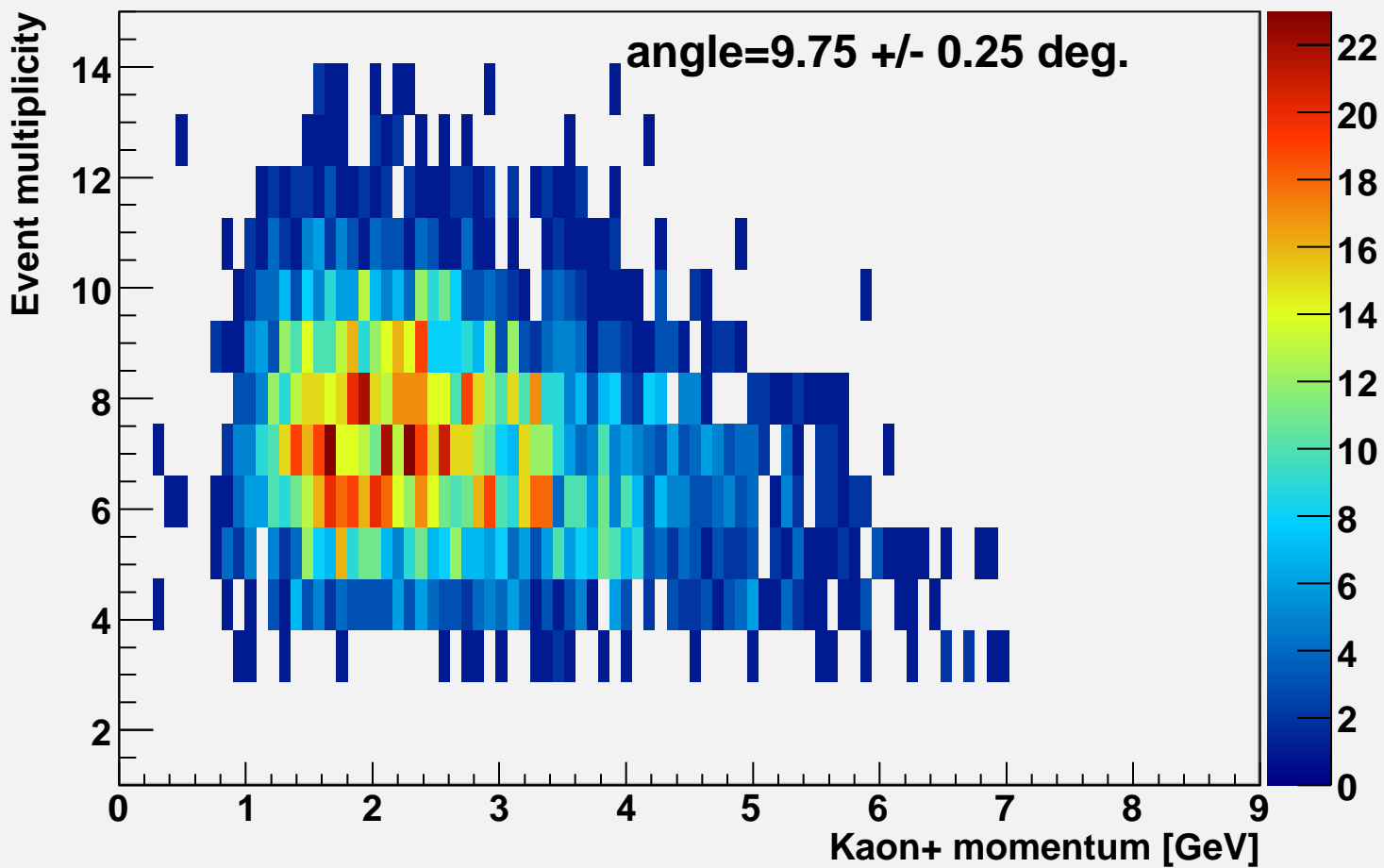
Event multiplicity vs k-momentum alpha=9.75
